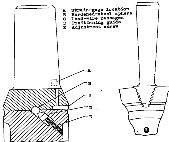
Figure 1. - Method of blade-root fastening used in investigation of vibration in loosely mounted turbine blades.
