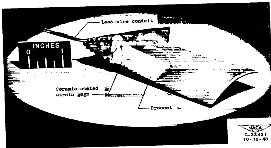
Figure 2. - High-temperature strain-gage instrumentation of turbine blade showing location of strain gage and lead-wire conduit.
