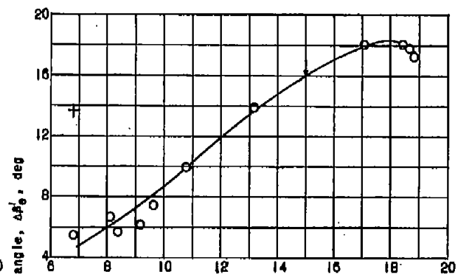
(c) Radial station c, \sigma = 0.822 .
