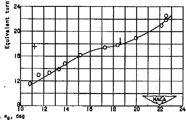
(d) Radial station d near hub, \sigma = 1.002 .
