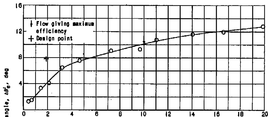
(a) Radial station a near tip, \sigma = 0.605 .
