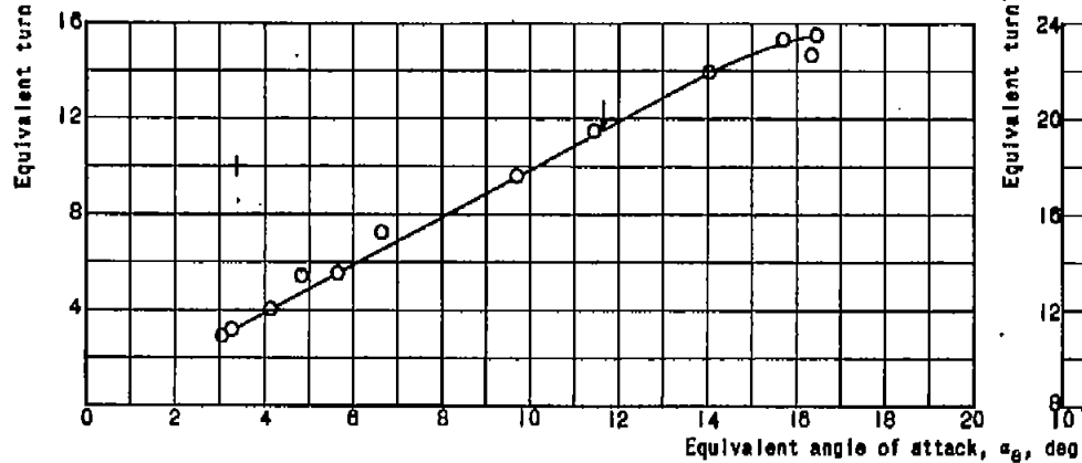
(b) Radial station b, \sigma = 0.696 .
