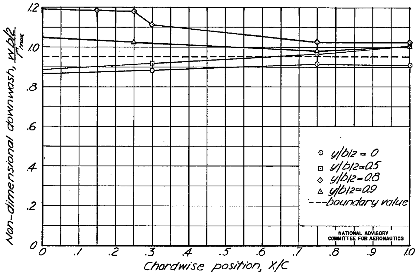
Figure 1.- Induced velocities calculated by the Cohen method for the loading predicted by the Falkner method on a 45° sweptback wing.
