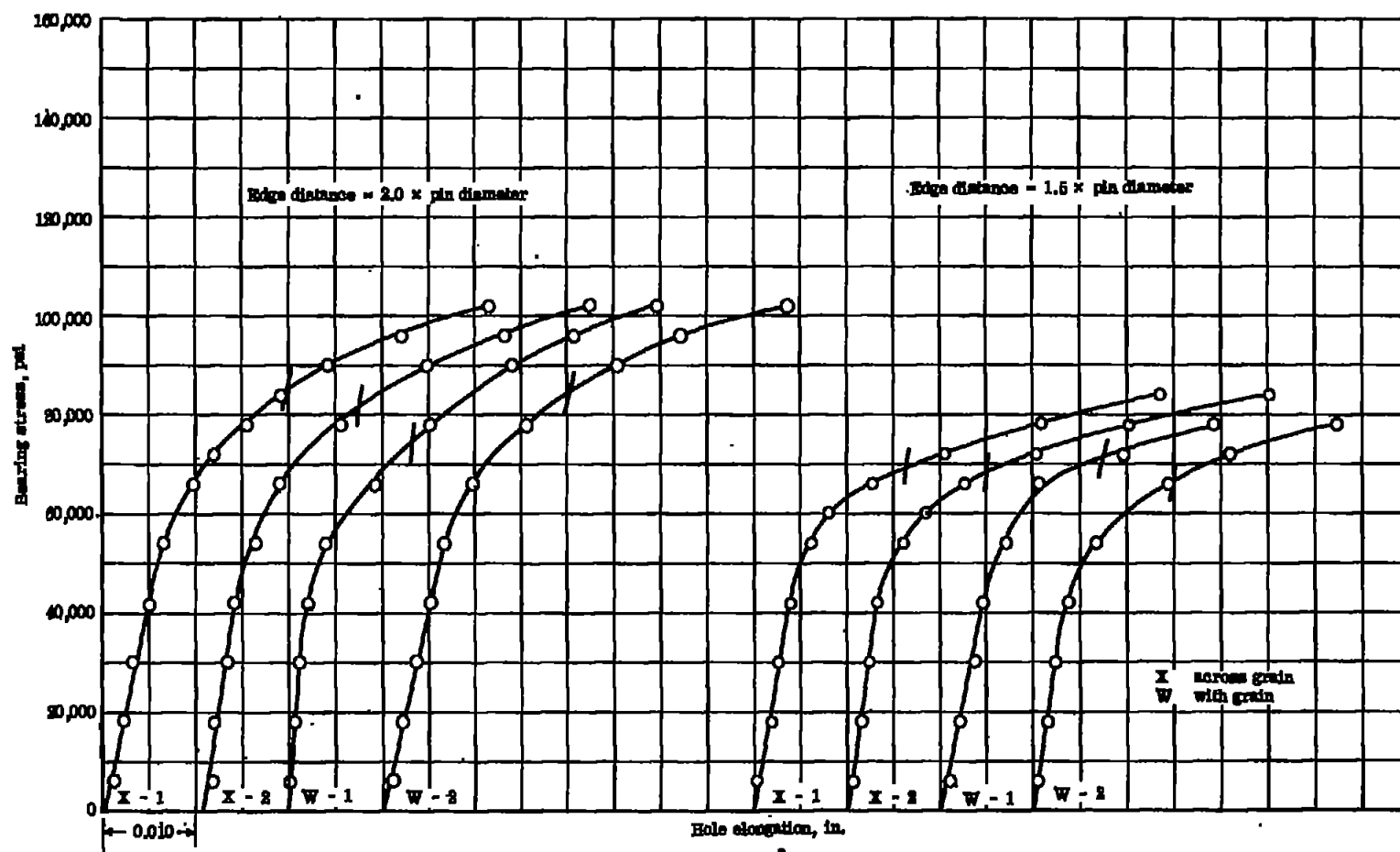
Figure 6.- Bearing stress-hole elongation curves for \frac{3}{4} -inch-thick 14S-W (annealed) plate. Specimen thickness, 0.250 inch; specimen width, 2 inches; pin diameter, 0.600 inch; bearing-yield offset, 0.03 \times pin diameter.
