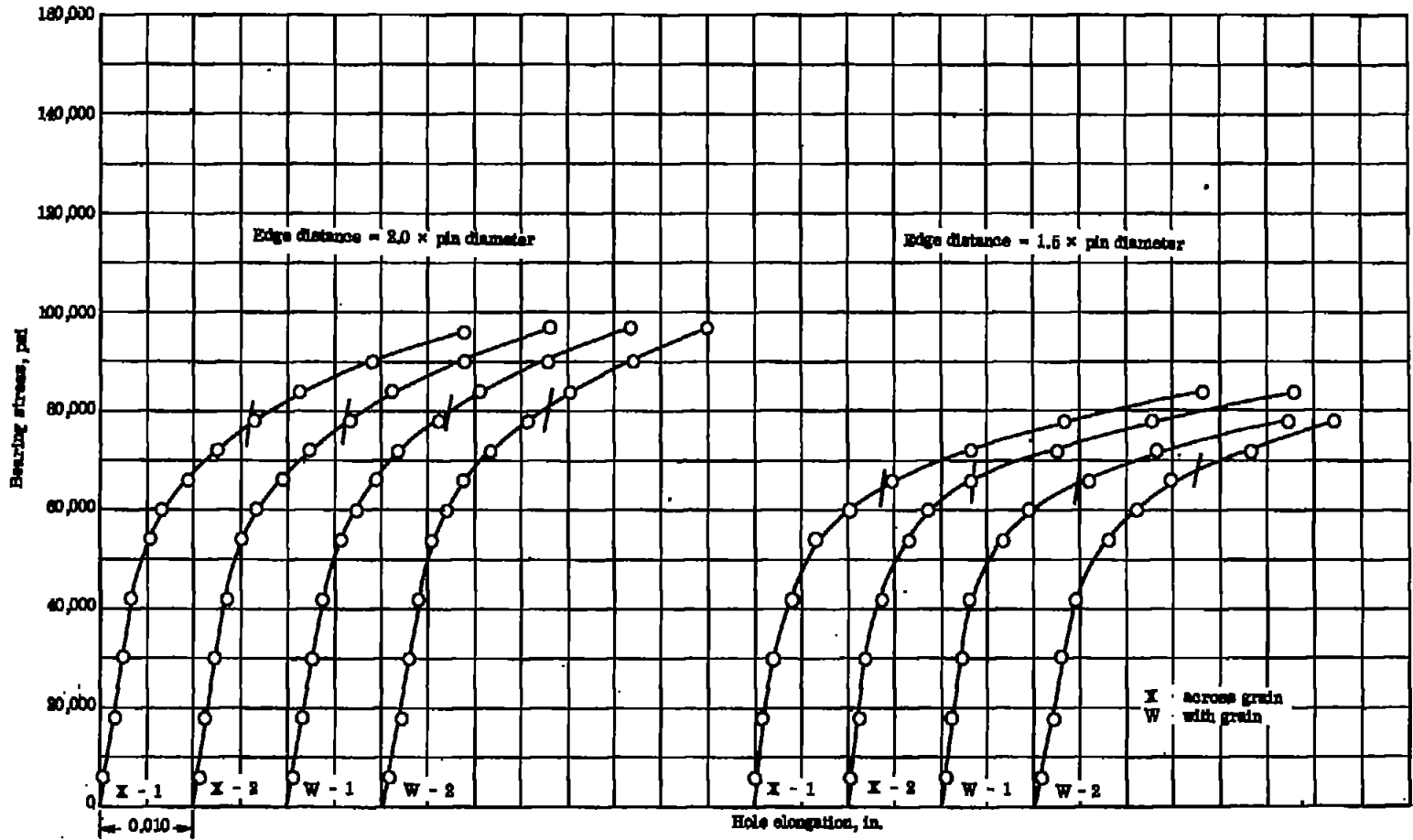
Figure 4.- Bearing stress-hole elongation curves for \frac{1}{4} -inch-thick Alclad 14S-W plate. Specimen thickness, 0.280 inch; specimen width, 2 inches; pin diameter, 0.500 inch; bearing-yield offset, 0.02 \times pin diameter,
