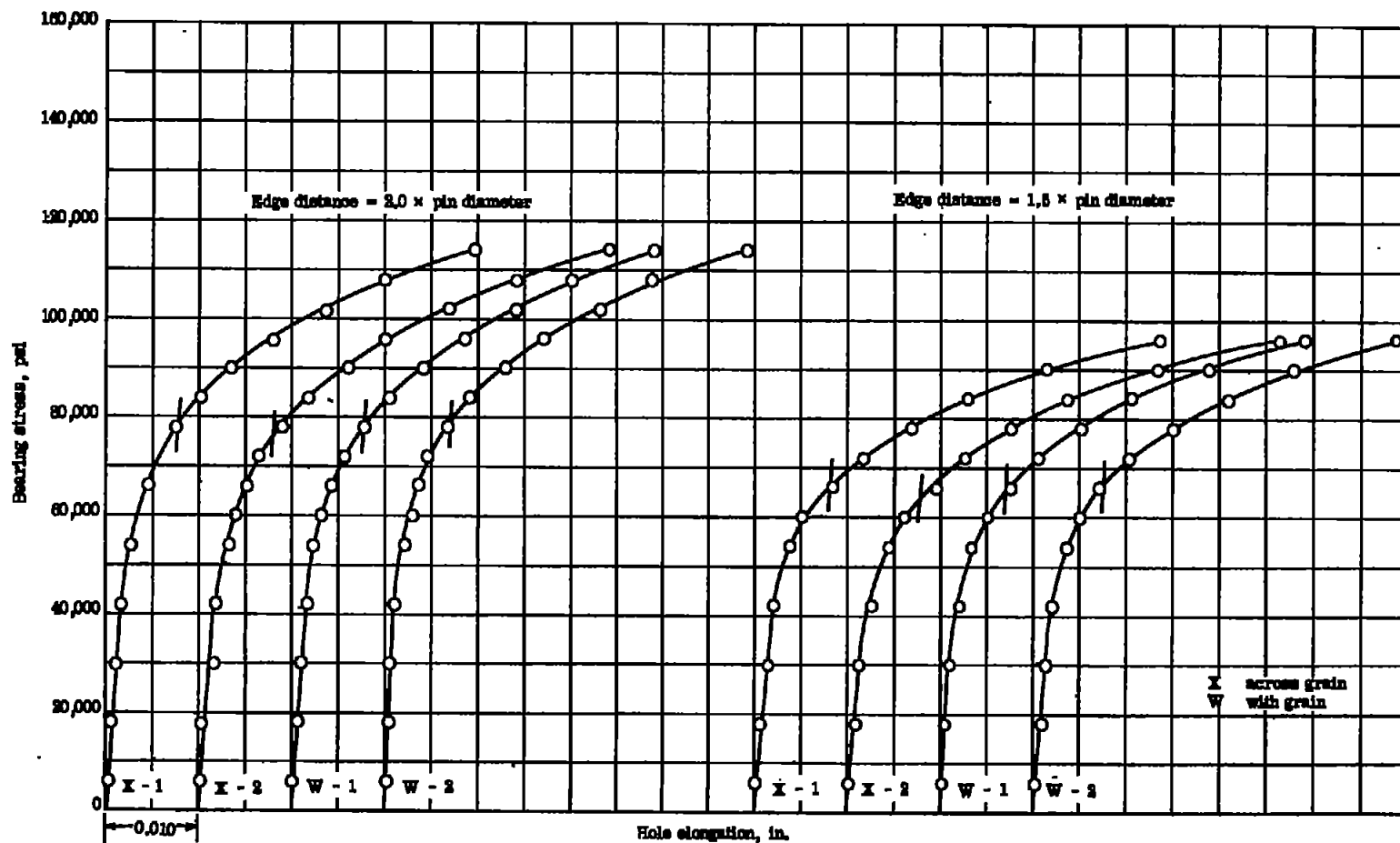
Figure 2.- Bearing stress-hole elongation curves for 0.064-inch-thick Alclad 14S-W sheet. Specimen thickness, 0.064 inch; specimen width, 2 inches; pin diameter, 0.380 inch; bearing-yield offset, 0.03 \times pin diameter.
