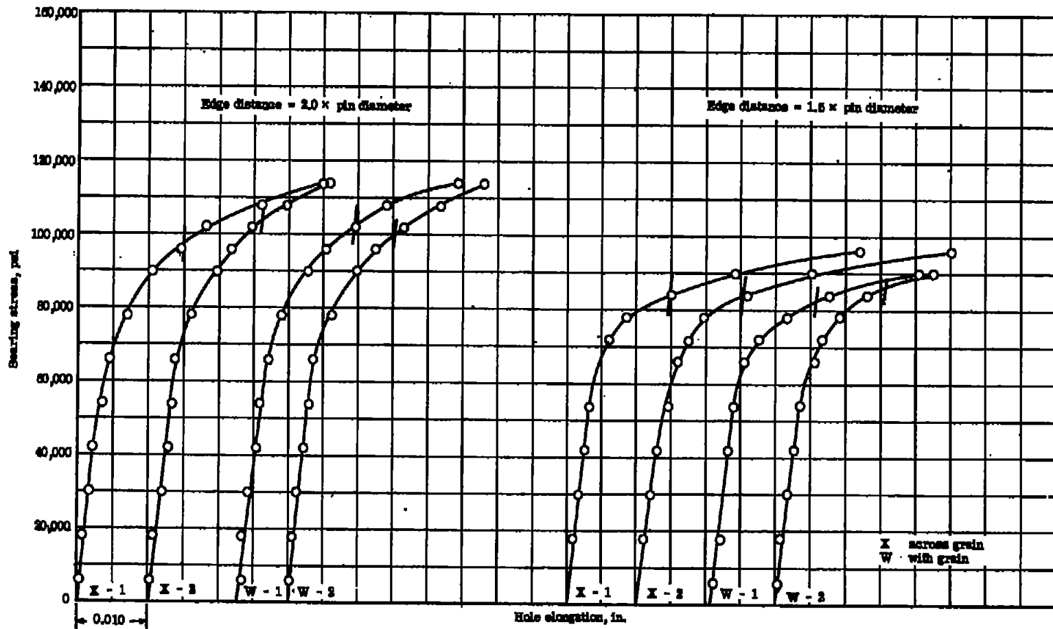
Figure 7.- Bearing stress-hole elongation curves for \frac{3}{4} -inch-thick 14S-T (normalized) plate. Specimen thickness, 0.250 inch; specimen width, 2 inches; pin diameter, 0.500 inch; bearing-yield offset, 0.02 \times pin diameter.
