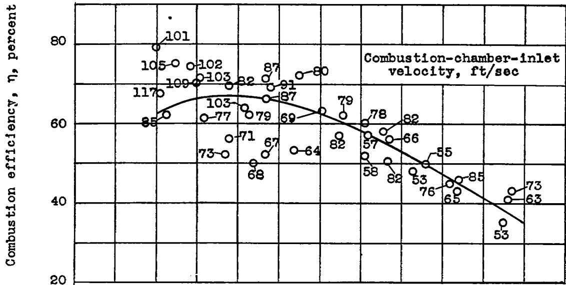
(c) Pressure altitude, 20,000 feet; combustion-chamber-inlet pressure, 1030 to 1130 pounds per square foot; average ambient-air temperature, 440° R.
