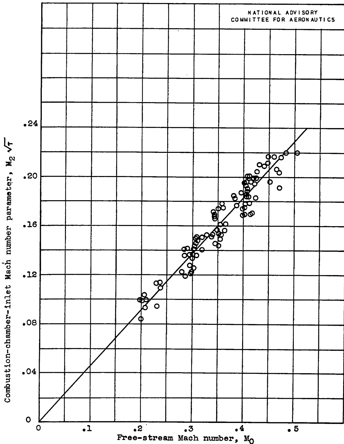
Figure 10. - Variation of combustion-chamber-inlet Mach number parameter with free-stream Mach number. 20-inch ram jet with 17-inch-diameter exhaust nozzle.
