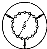
View A Fuel-spray manifold
