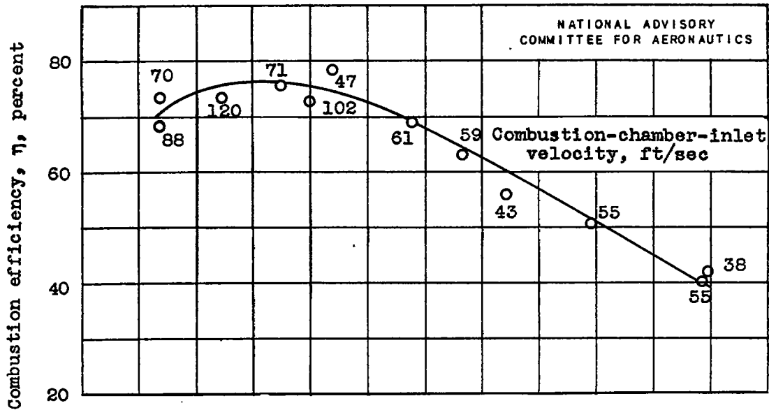
(a) Pressure altitude, 5000 feet; combustion-chamber-inlet pressure, 1780 to 1865 pounds per square foot; average ambient-air temperature, 472° R.
