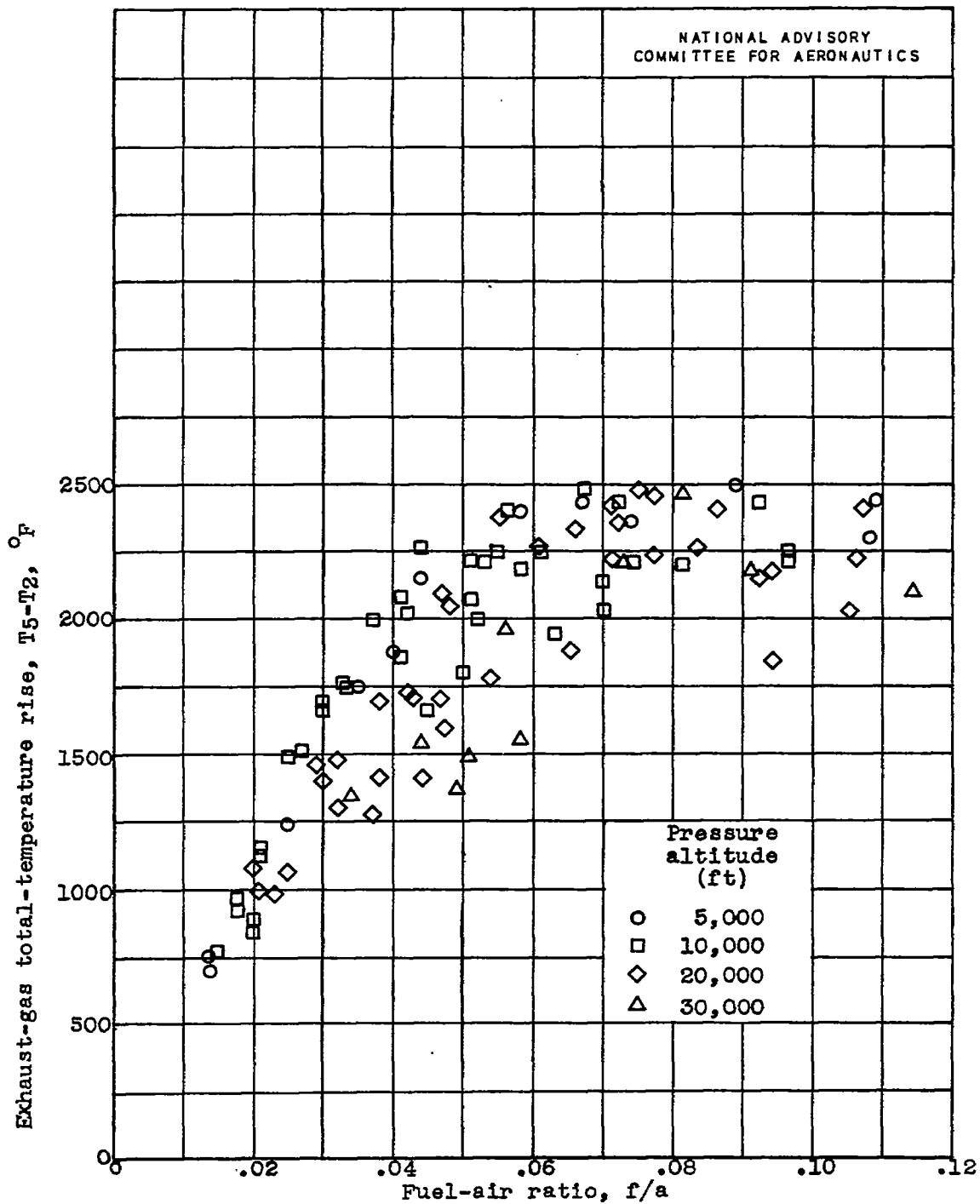
Figure 5. - Variation of exhaust-gas total-temperature rise with fuel-air ratio and altitude. 20-inch ram jet with 17-inch-diameter exhaust nozzle.
