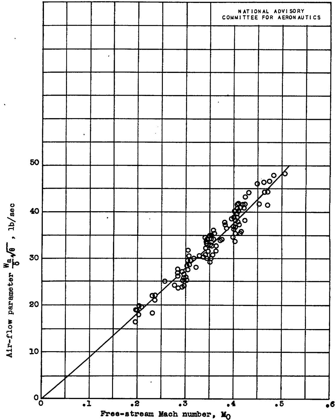
Figure 11. - Variation of air-flow parameter with free-stream Mach number. 20-inch ram jet with 17-inch-diameter exhaust nozzle.
