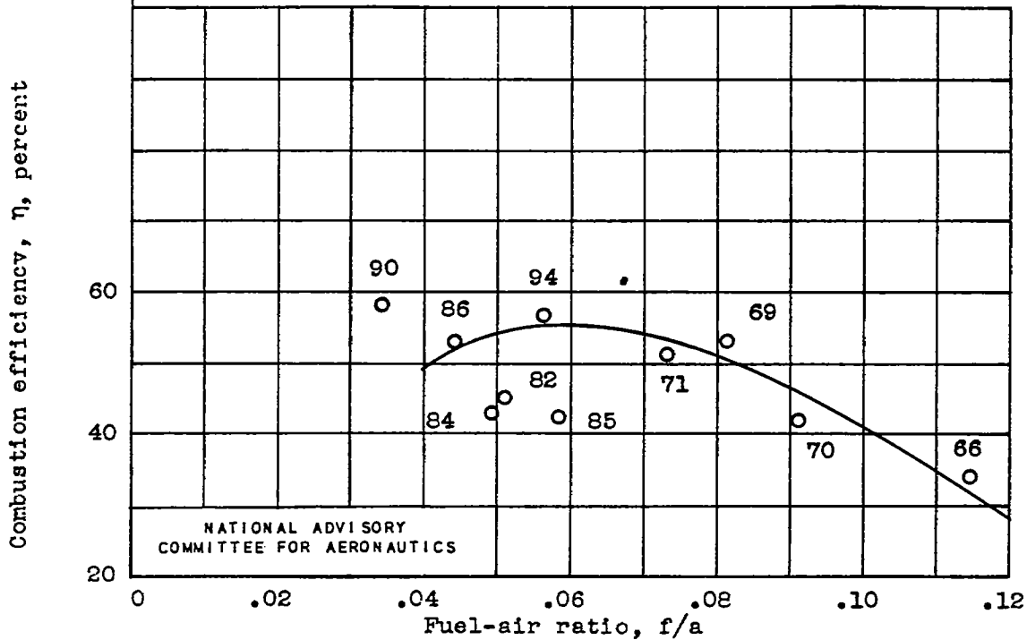
(d) Pressure altitude, 30,000 feet; combustion-chamber-inlet pressure, 690 to 760 pounds per square foot; average ambient-air temperature, 410° R.
