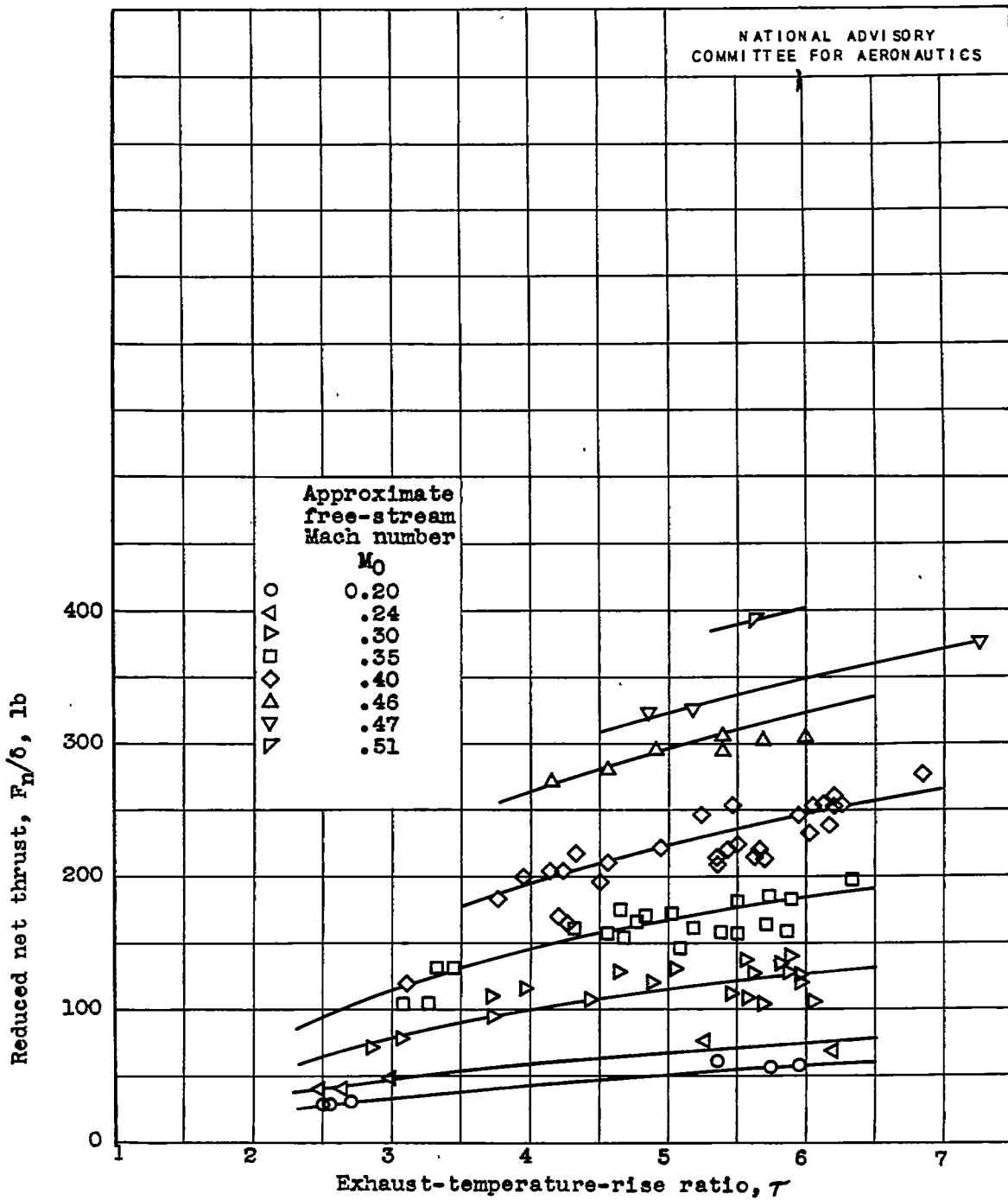
Figure 12. - Variation of reduced net thrust with exhaust-temperature-rise ratio and approximate free-stream Mach number. 20-inch ram jet with 17-inch-diameter exhaust nozzle.
