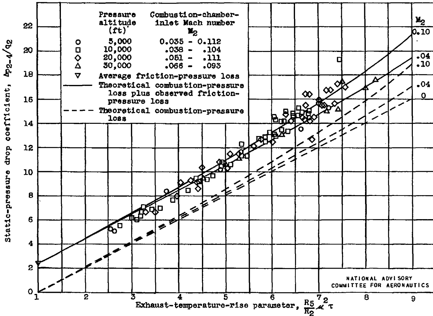
Figure 9. - Variation of measured static-pressure drop coefficient with exhaust-temperature rise parameter and combustion-chamber-inlet Mach number. 20-inch ram jet with 17-inch-diameter exhaust nozzle.
