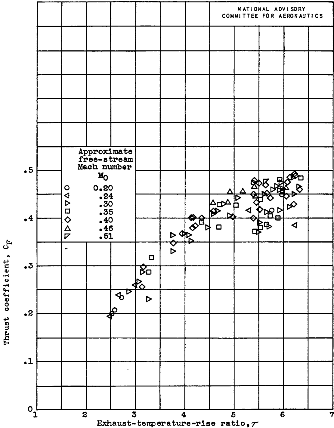
Figure 14. - Effect of exhaust-temperature-rise ratio and free-stream Mach number on thrust coefficient. 20-inch ram jet with 17-inch-diameter exhaust nozzle.
