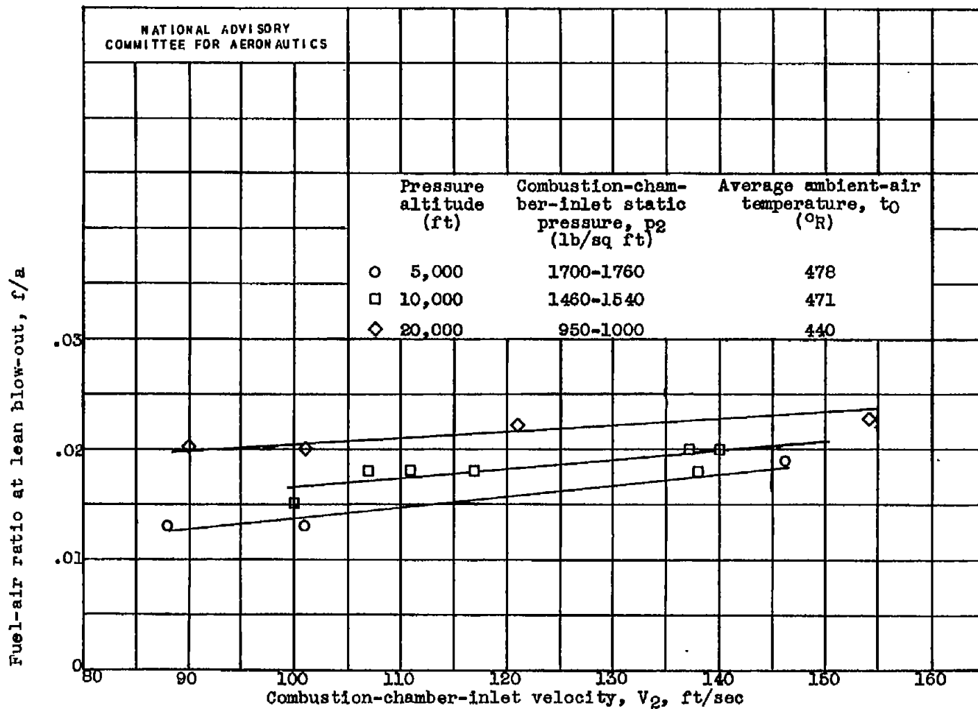
Figure 4. - Variation of fuel-air ratio at lean blow-out with combustion-chamber-inlet velocity for various pressure altitudes. 20-inch ram jet with 17-inch-diameter exhaust nozzle.
