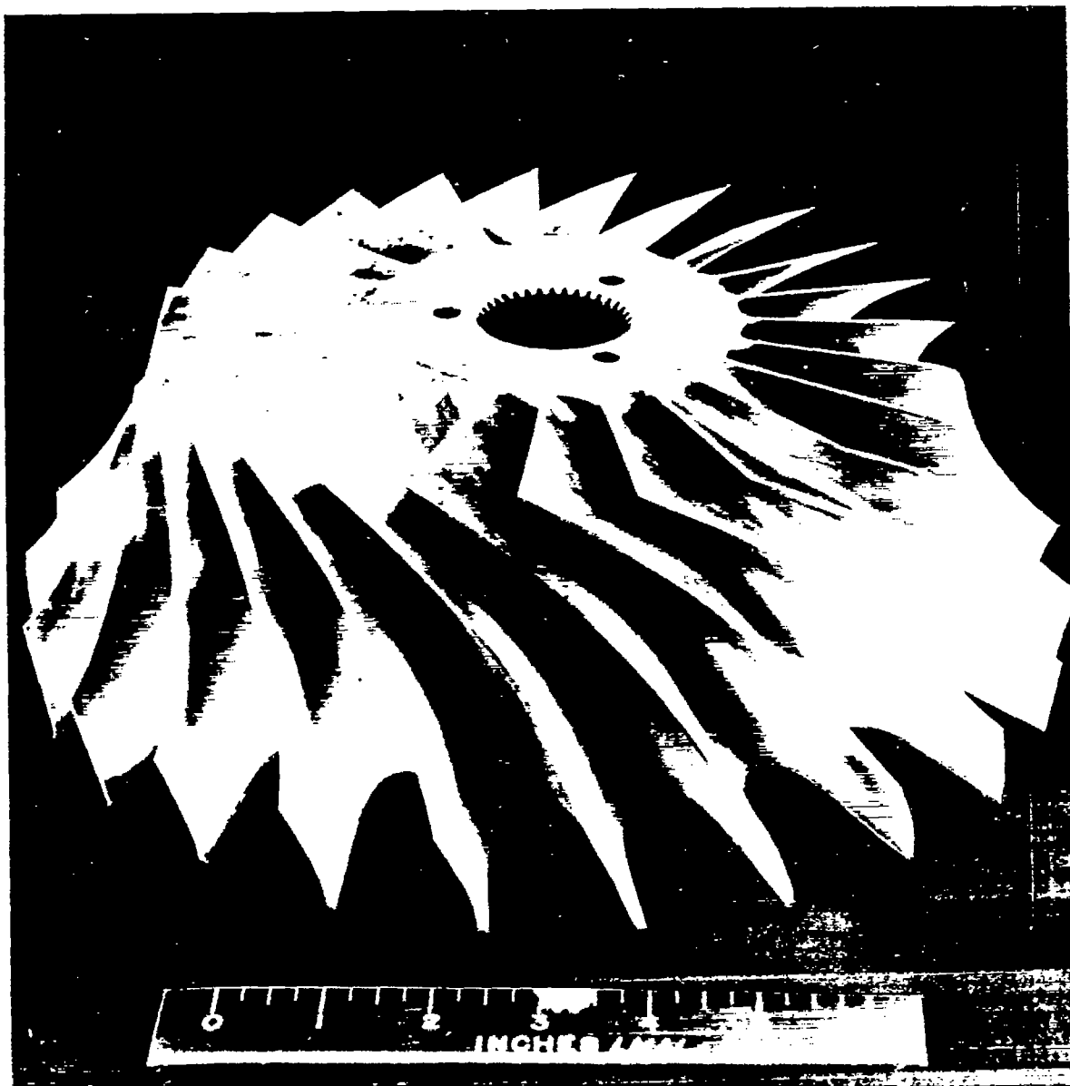
Figure 2. - Mixed-flow impeller B.
