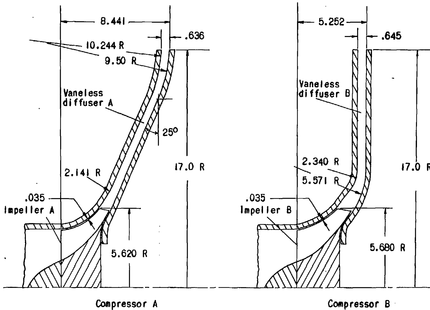
Figure 1. - Dimensional comparison of passage curvature in vaneless diffusers A and B. (All dimensions in in.)
