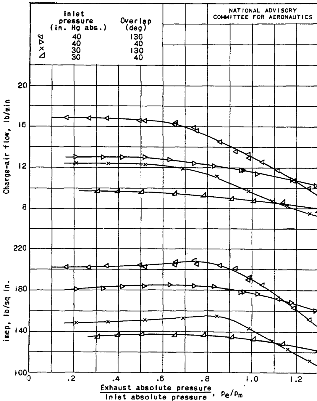
Figure 4. - Concluded. Variation of indicated mean effective pressure and charge-air flow with ratio of exhaust absolute pressure to inlet absolute pressure.
