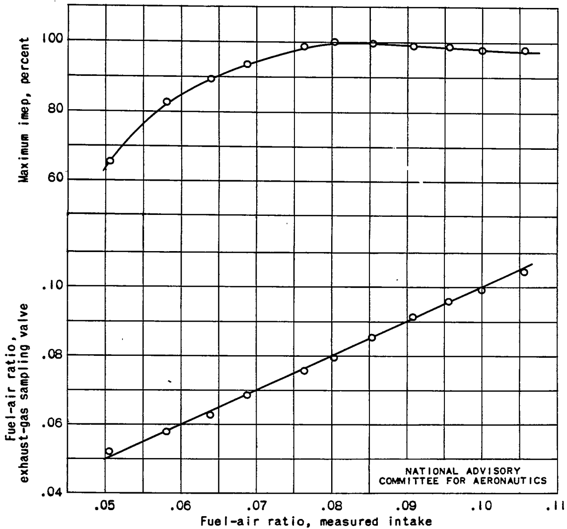
Figure 3. - Accuracy of exhaust-gas sampling valve and percentage change in power output with fuel-air ratio. Valve overlap, 40°; inlet-manifold pressure, 35 inches mercury absolute; exhaust pressure, 35 inches mercury absolute; engine speed, 2000 rpm; combustion-air temperature, 200° F.
