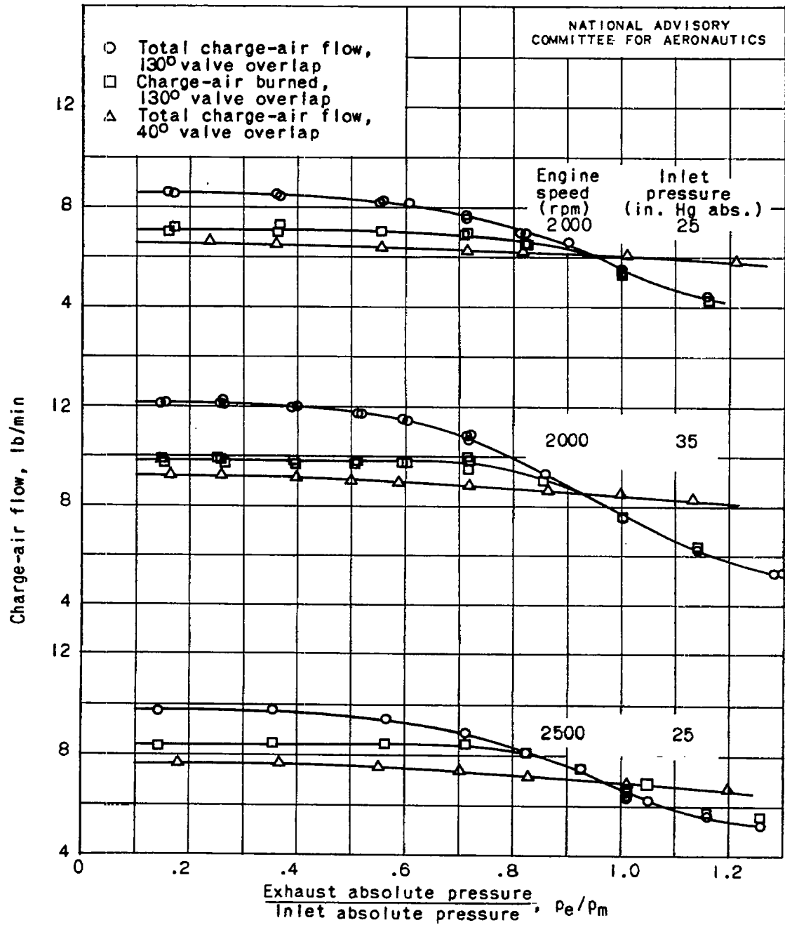
Figure 6. - Utilization of charge-air flow with 130° valve overlap determined from combustion-gas samples.
