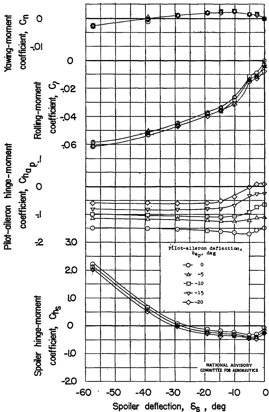
(b) \alpha = 12.3^\circ ; full-span double slotted flaps deflected 50^\circ .
