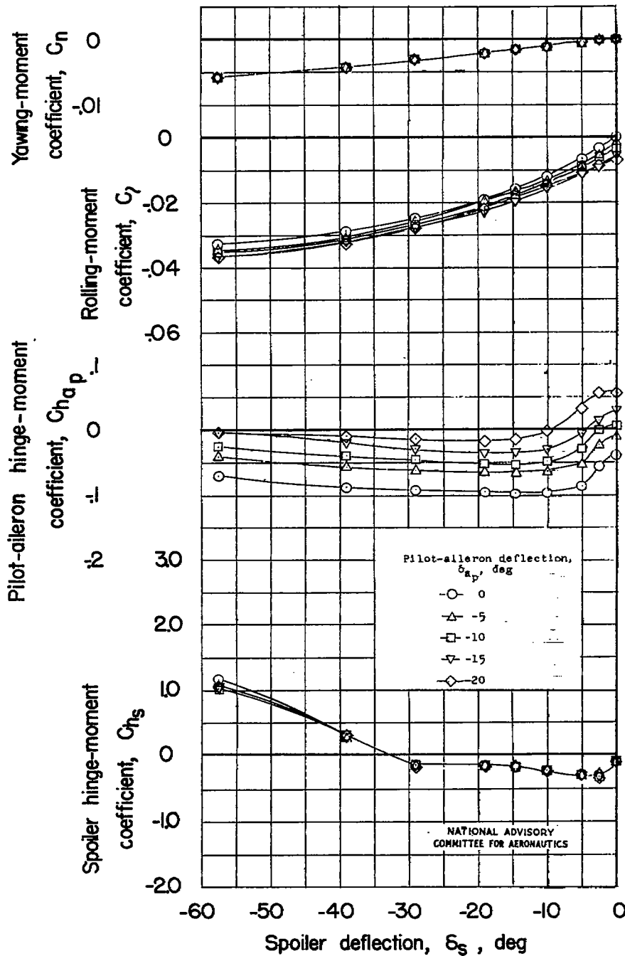
(a) \alpha = 3.5^\circ ; flaps neutral.
