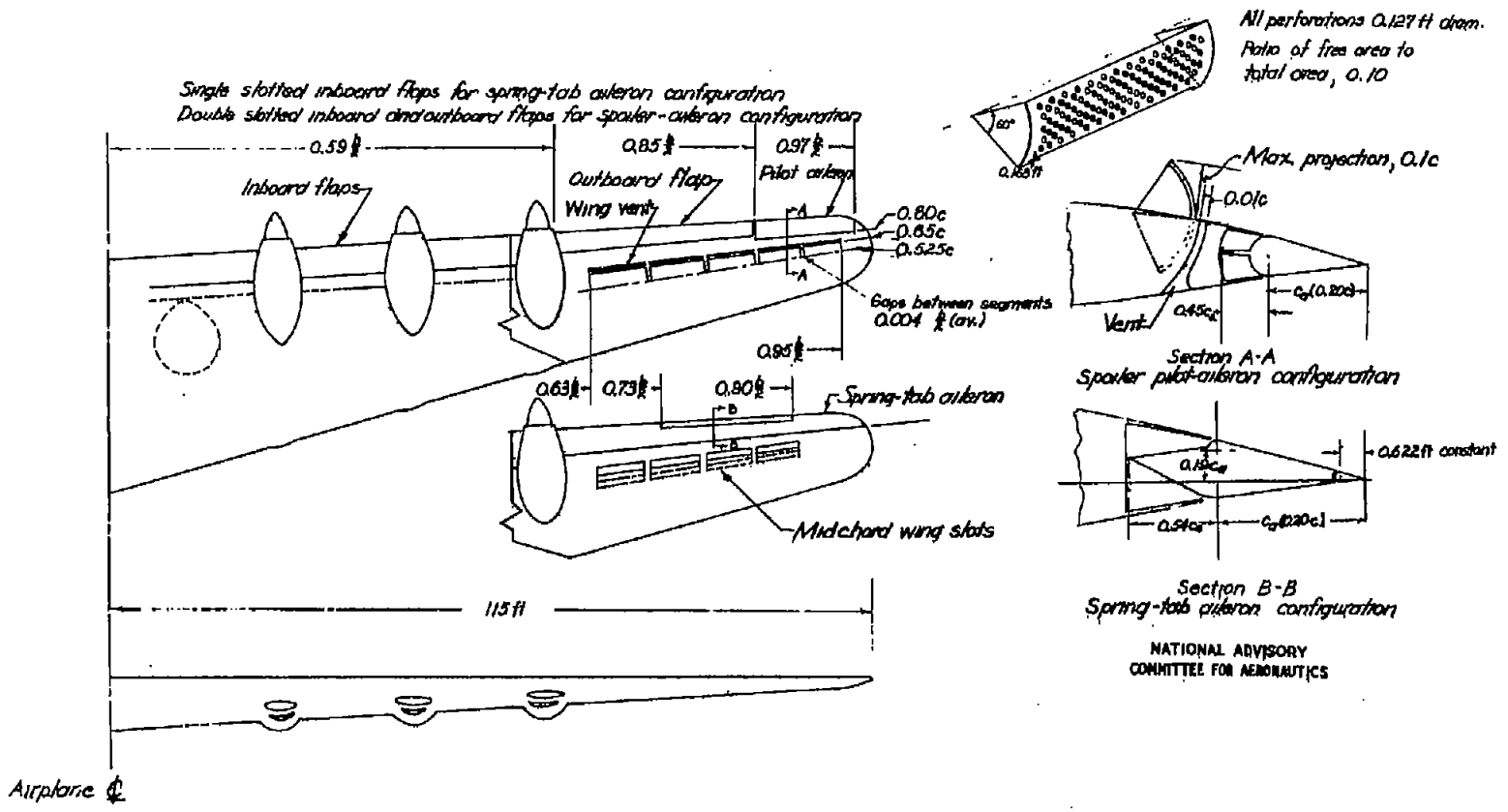
Figure 1.- Geometric characteristics of the wing and lateral-control systems.
