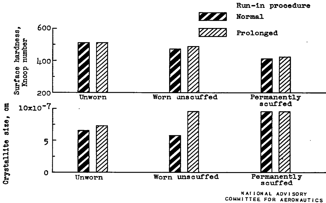
Figure 9. - Relation between surface changes and surface condition of cast-iron slider specimens.
