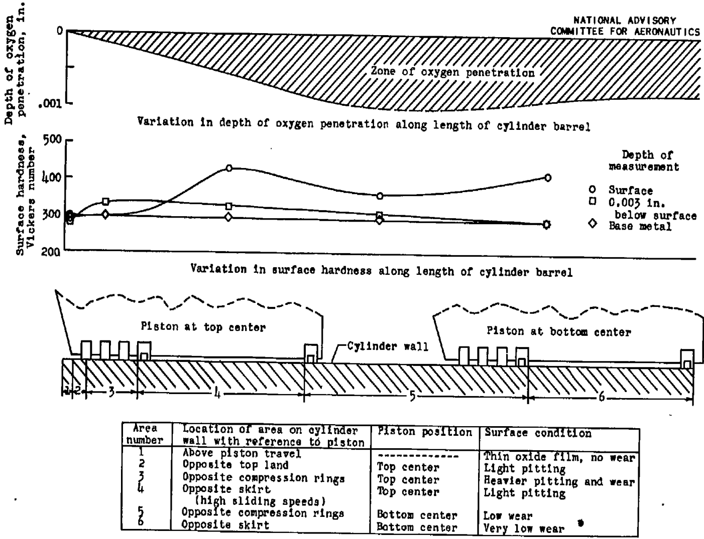
Figure 6. - Relations among surface condition, material hardness, and depth of oxygen penetration found on worn - unscuffed SAE 4140 steel aircraft-engine cylinder barrel.
