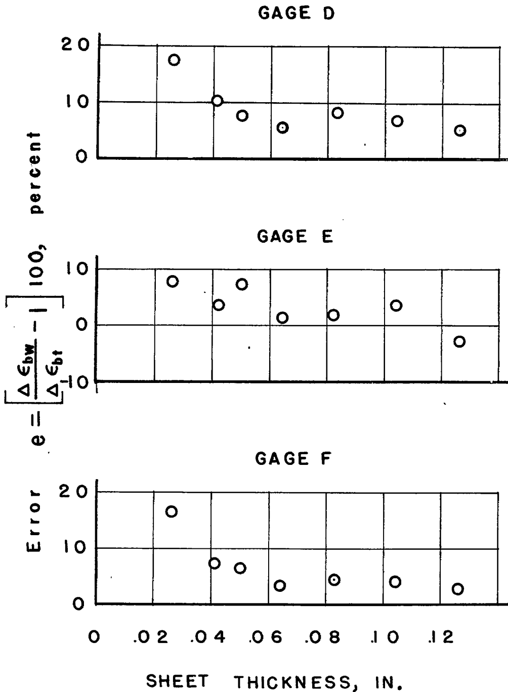
Figure 3.- Average error in the extreme-fiber strain, indicated by wire gages D, E, and F, plotted against sheet thickness.
