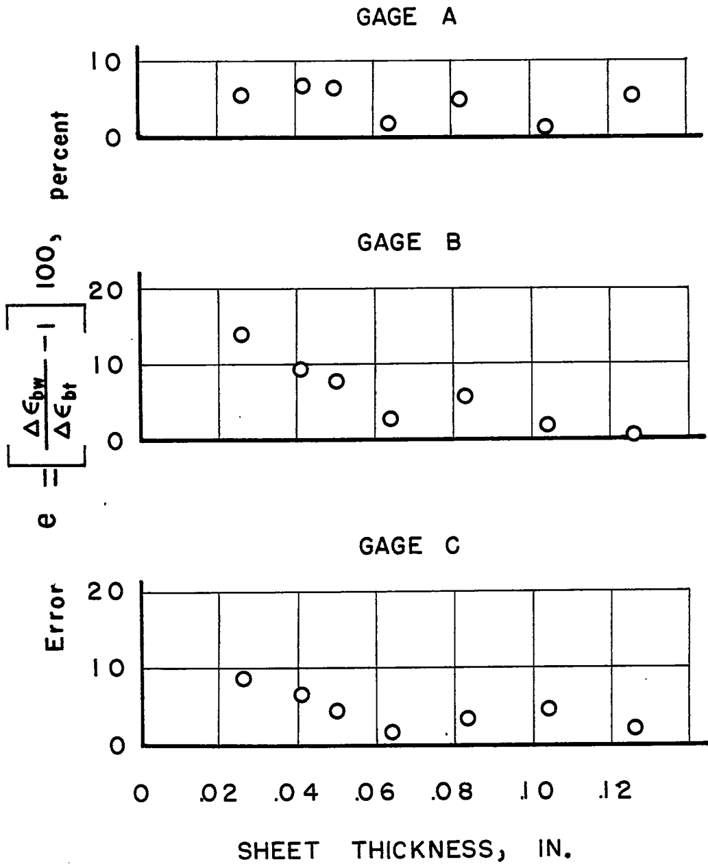
Figure 2.- Average error in the extreme-fiber strain, indicated by wire gages A, B, and C, plotted against sheet thickness.
