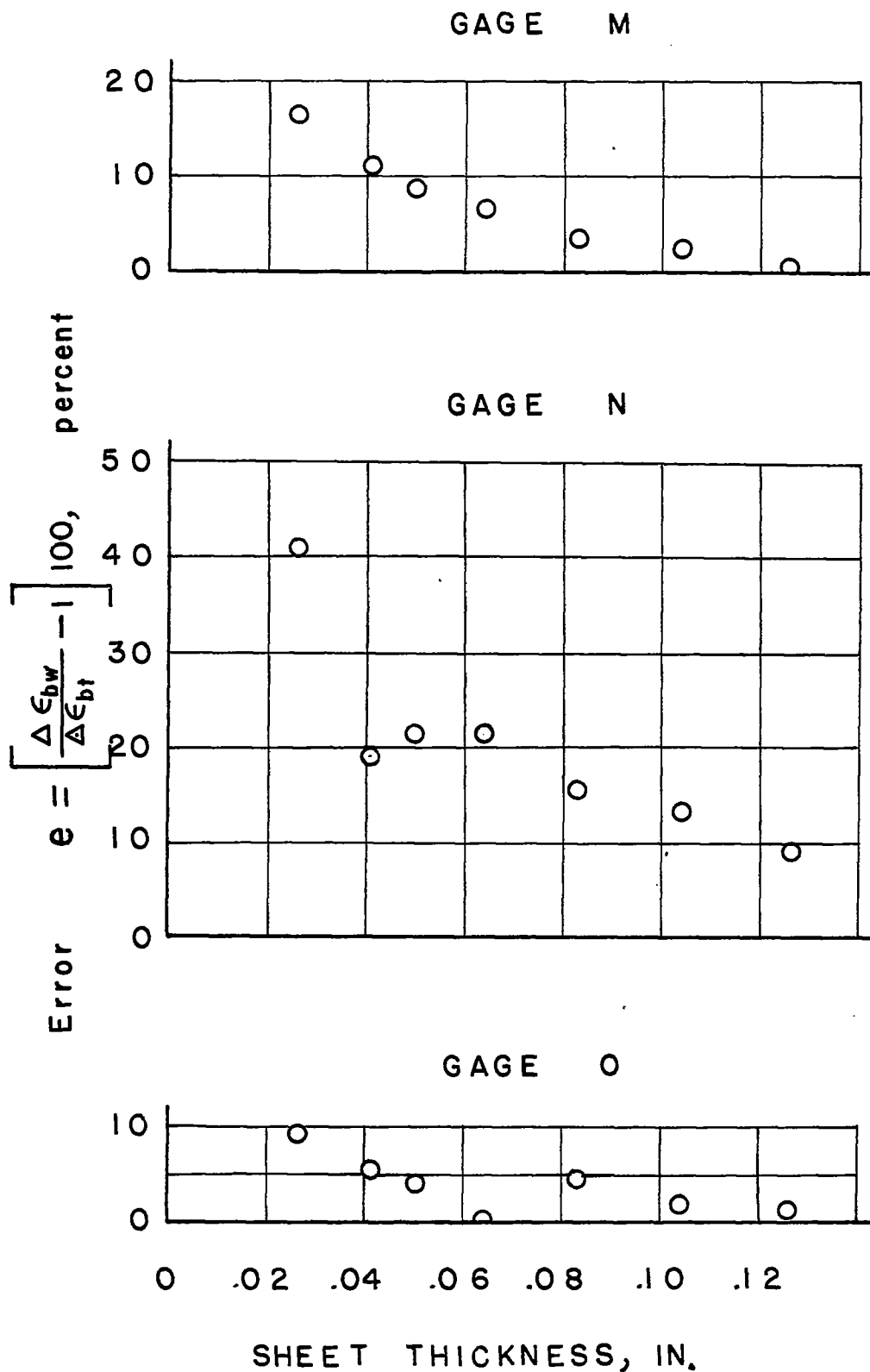
Figure 6.- Average error in the extreme-fiber strain, indicated by wire gages M, N, and O, plotted against sheet thickness.
