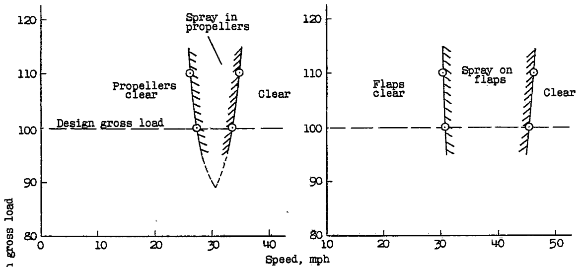
(a) 145,000-pound cargo flying boat. Flap deflection, 30°.
