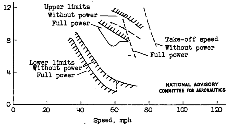
(c) 26,000-pound amphibian. Flap deflection, 20°.
