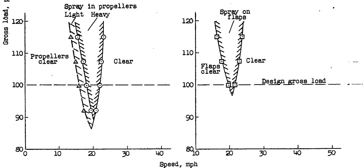
(b) 26,000-pound amphibian. Flap deflection, 0°.
