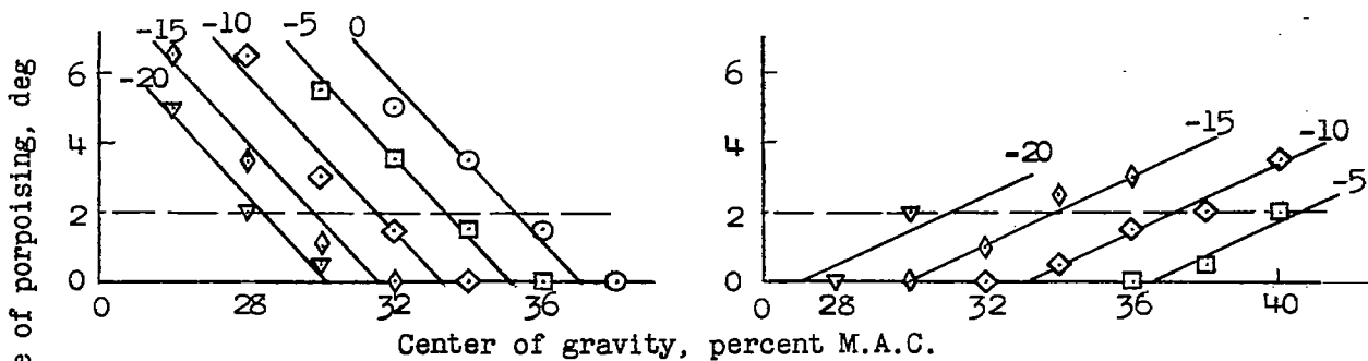
(b) 145,000-pound cargo flying boat. Flap deflection, 30°.
