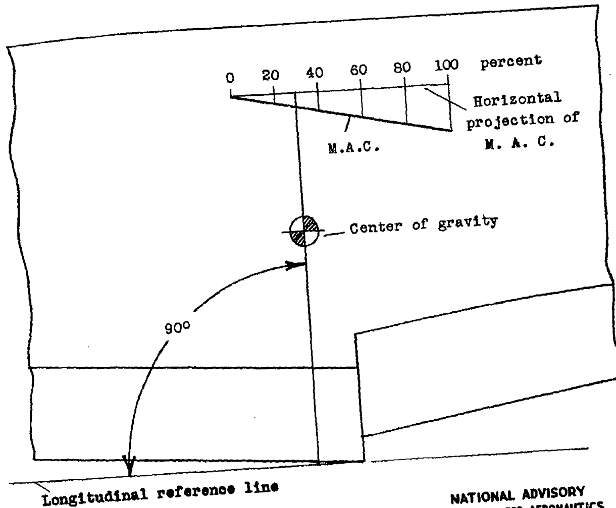
Figure 2.- Standard definition of longitudinal position of center of gravity in percent of the M.A.C. Center of gravity shown is 30 percent M.A.C.
