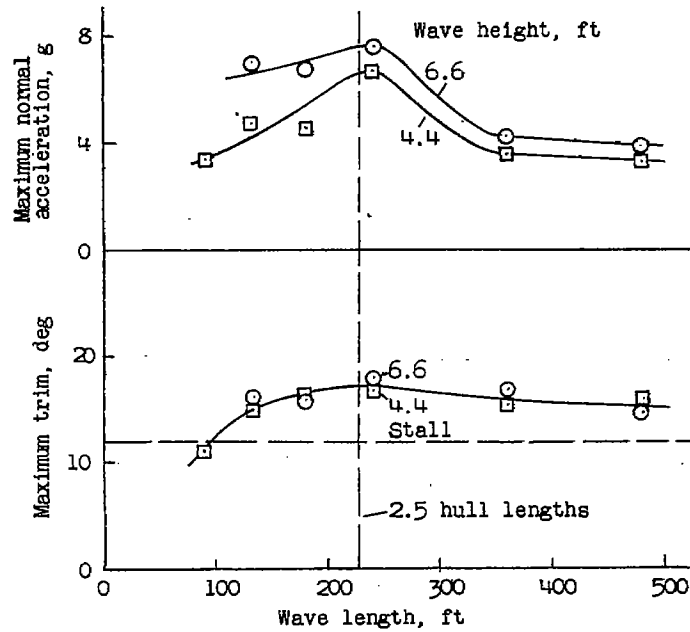
(a) 145,000-pound cargo flying boat.
