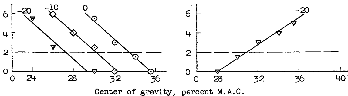
(c) 20,000-pound amphibian. Flap deflection, 20°.
