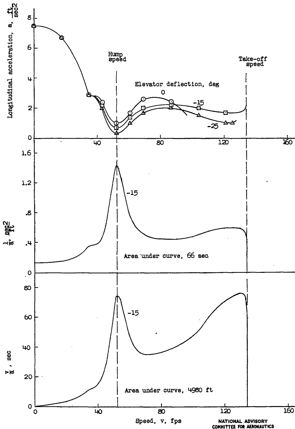
Figure 9.- Typical variation of longitudinal acceleration a , 1/a , and v/a with speed during take-off. 165,000-pound cargo flying boat; wing loading, 45 pounds per square foot; power loading, 14 pounds per horsepower.
