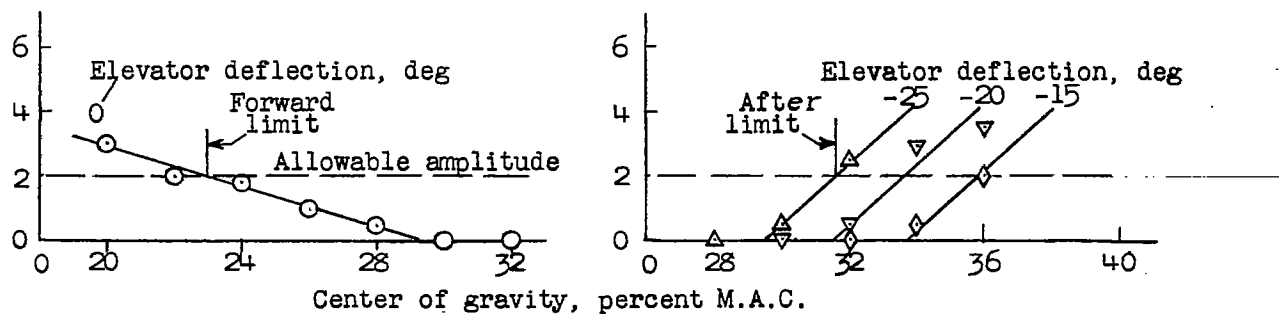
(a) 400,000-pound cargo flying boat. Flap deflection, 20°.
