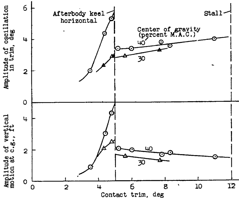
(b) 145,000-pound cargo flying boat.
