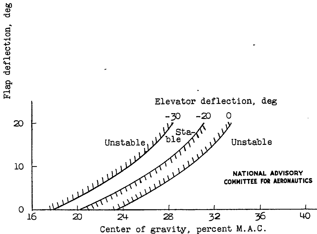
(a) 75,000-pound patrol-bomber flying boat.
