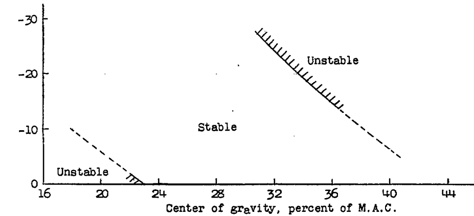
(a) 400,000-pound cargo flying boat. Flap deflection, 20°.
