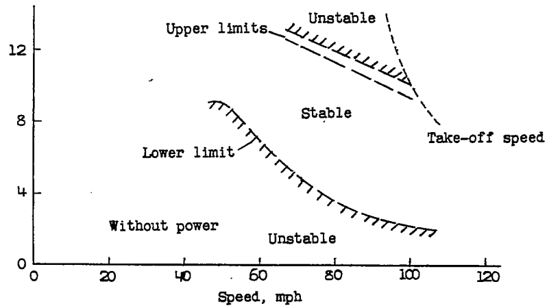
(a) 400,000-pound cargo flying boat. Flap deflection, 20°.
