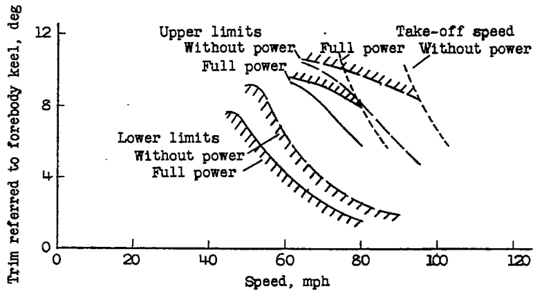
(b) 145,000-pound cargo flying boat. Flap deflection, 30°.
