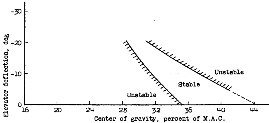
(a) 400,000-pound cargo flying boat. Flap deflection, 20°.
