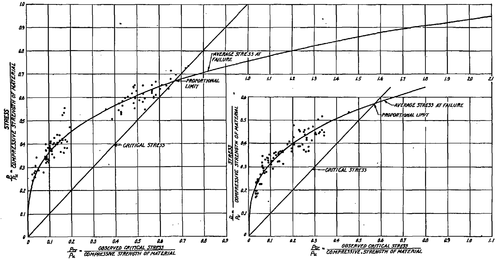
Figure 4.-Plywood plates in compression. Compressive stress parallel to face grain. (Same data as in fig. 2.)
