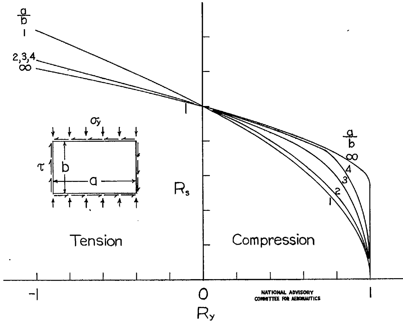
Figure 5.- Transition in the form of interaction curve for shear and transverse direct stress for a simply supported rectangular flat plate as the length-width ratio changes from 1 to \infty in terms of
