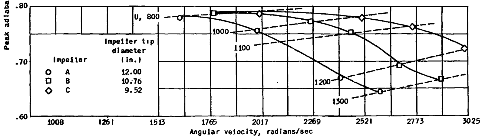
(b) Impellers.
