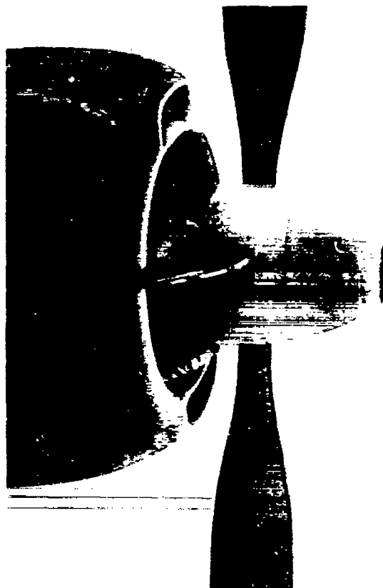
Figure 9.- Ice accretion on leading edge of air-heated propeller after flight in light-icing conditions.
