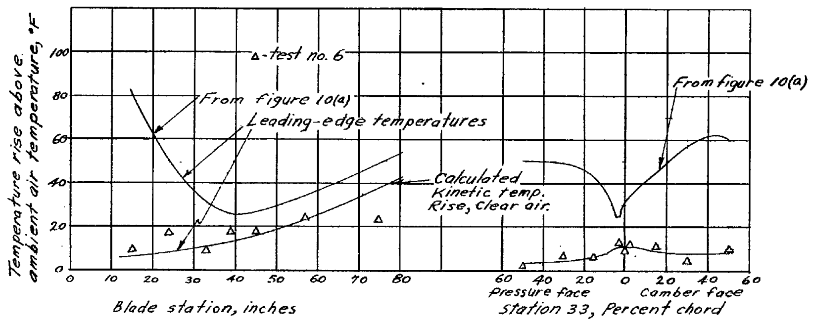
(b) Comparison of (a) with clear air, unheated air flow to propeller
