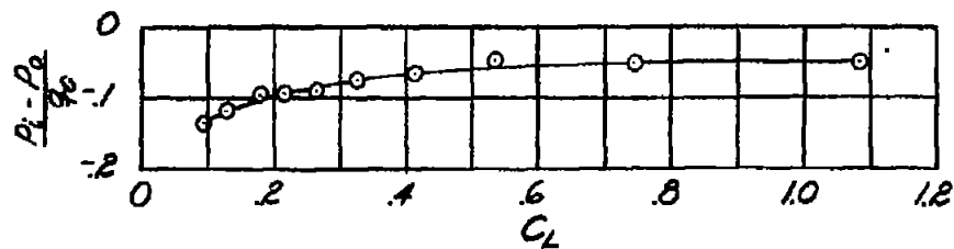
(a) Variation of \frac{P_i - P_o}{q_c} with C_L from unaccelerated-flight data.
