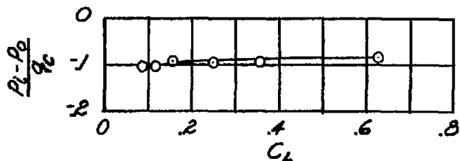
(a) Variation of \frac{p_1 - p_0}{q_c} with C_L from unaccelerated-flight data.
