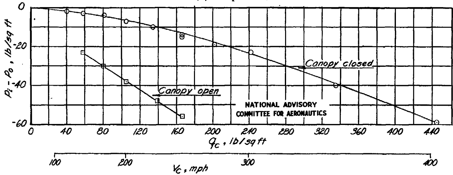
(e) Airplane E.
