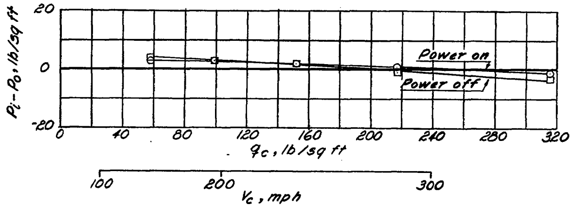
(b) Airplane B; canopy closed.
