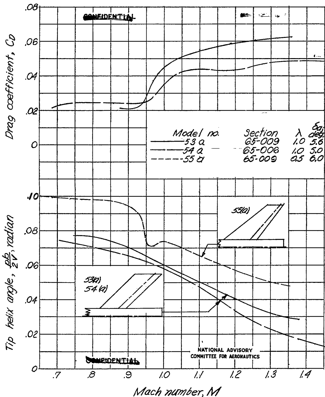
Figure 6 .- Effect of thickness and taper on the variation of tip helix angle and drag coefficient with Mach number. A=3.0 ; \alpha = 45 deg. Data for model 53a from reference 1.
