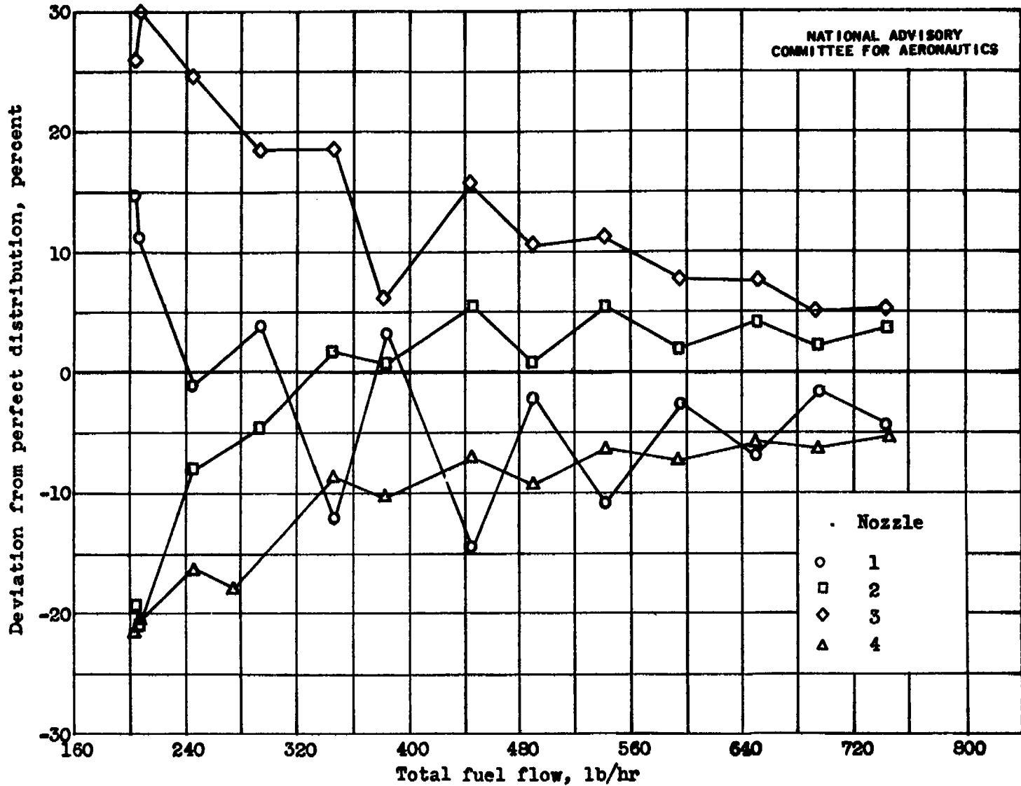
Figure 8. - Deviation from perfect distribution at various fuel flows of spring-loaded nozzles connected to manifold.
