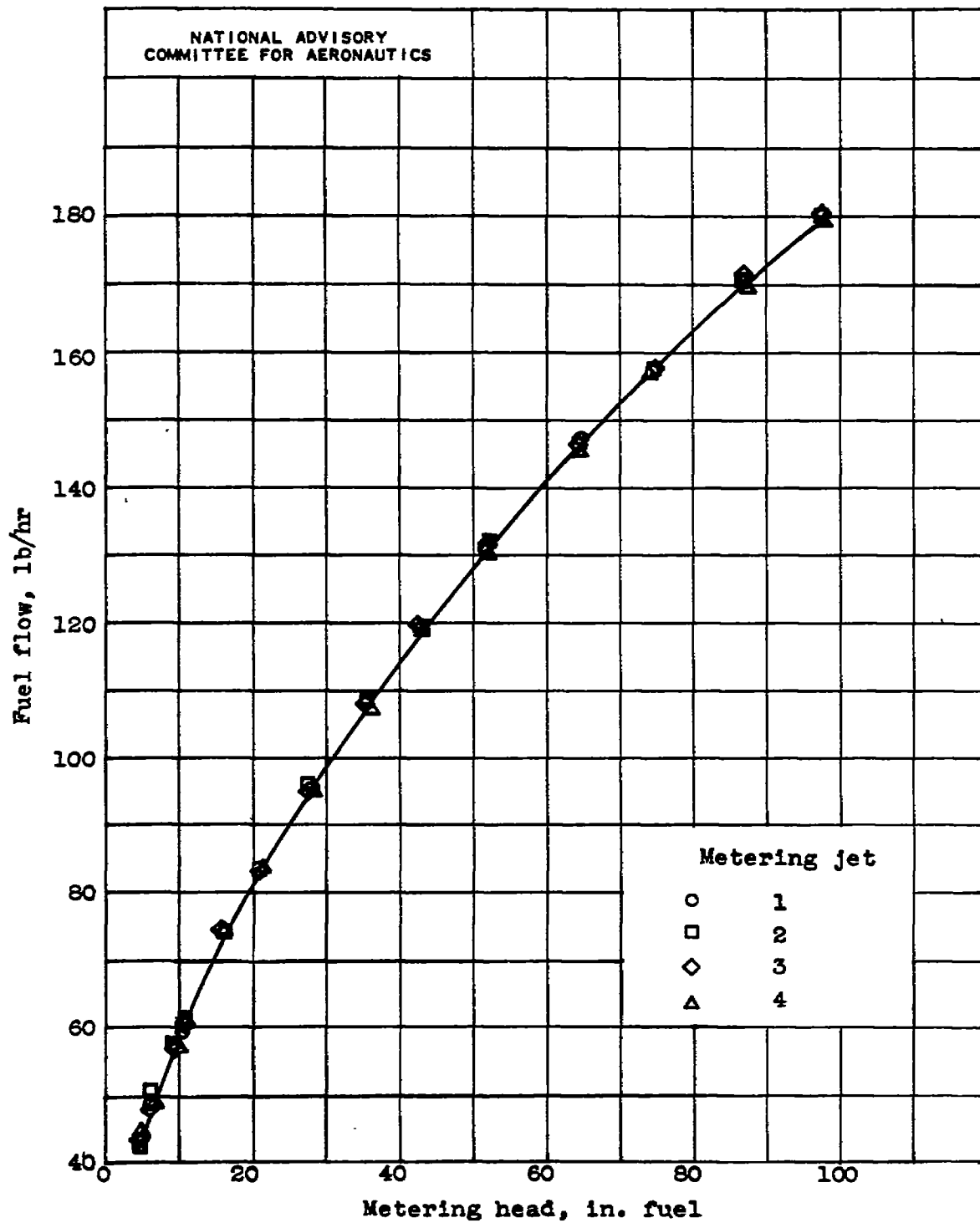
Figure 4. - Variation of fuel flow with metering head for matched metering jets used in experimental model of fuel-distribution control. Fuel specific gravity, 0.74 at 70° F.
