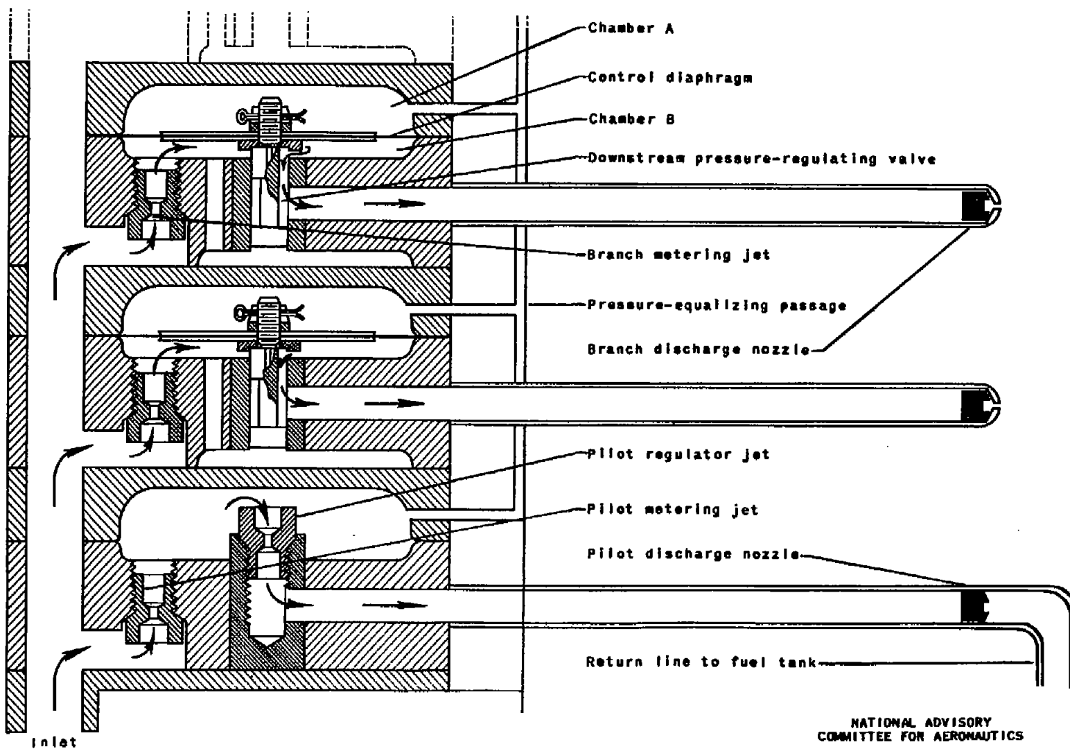
Figure 2. - Schematic diagram of fuel-distribution control for continuous-flow manifold injection.
