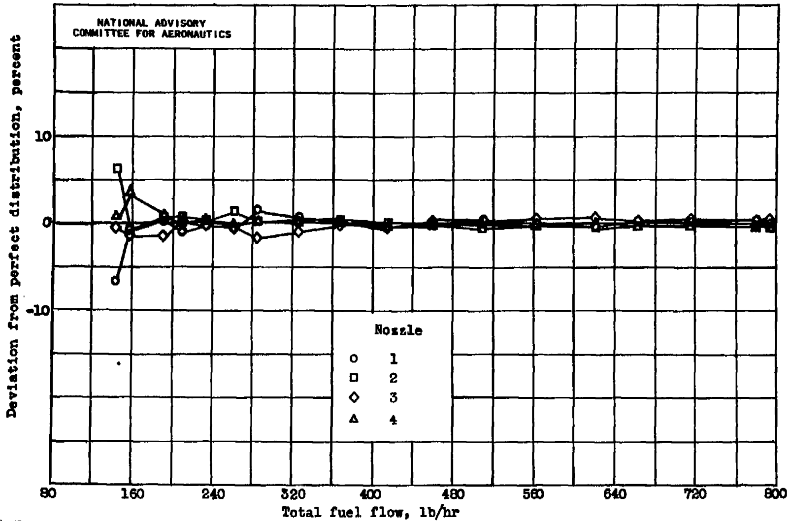
Figure 9. - Deviation from perfect distribution at various fuel flows of spring-loaded nozzles connected to experimental model of fuel-distribution control.
