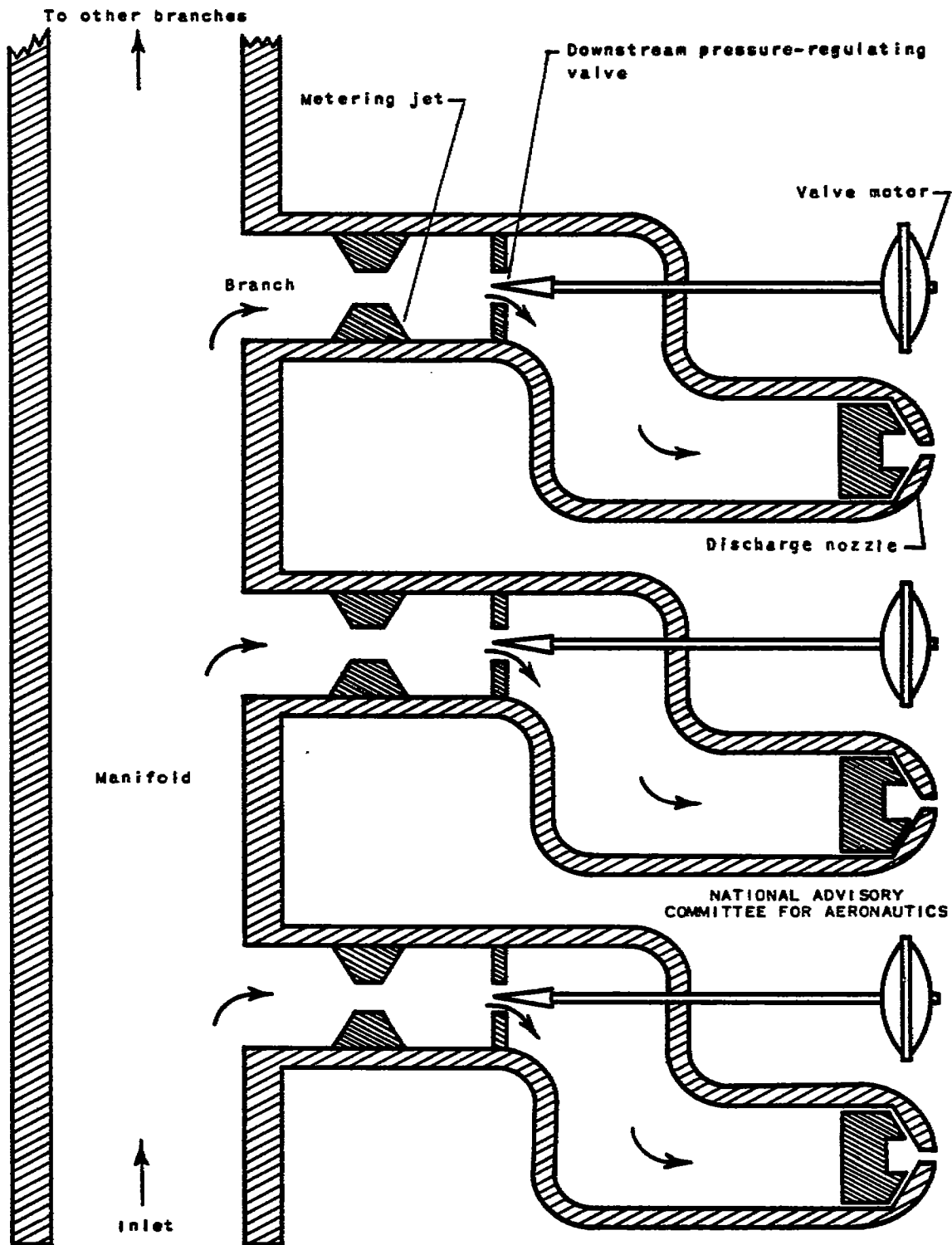
Figure 1. - Schematic diagram of control elements in apparatus for maintaining equal fuel distribution to unmatched nozzles.
