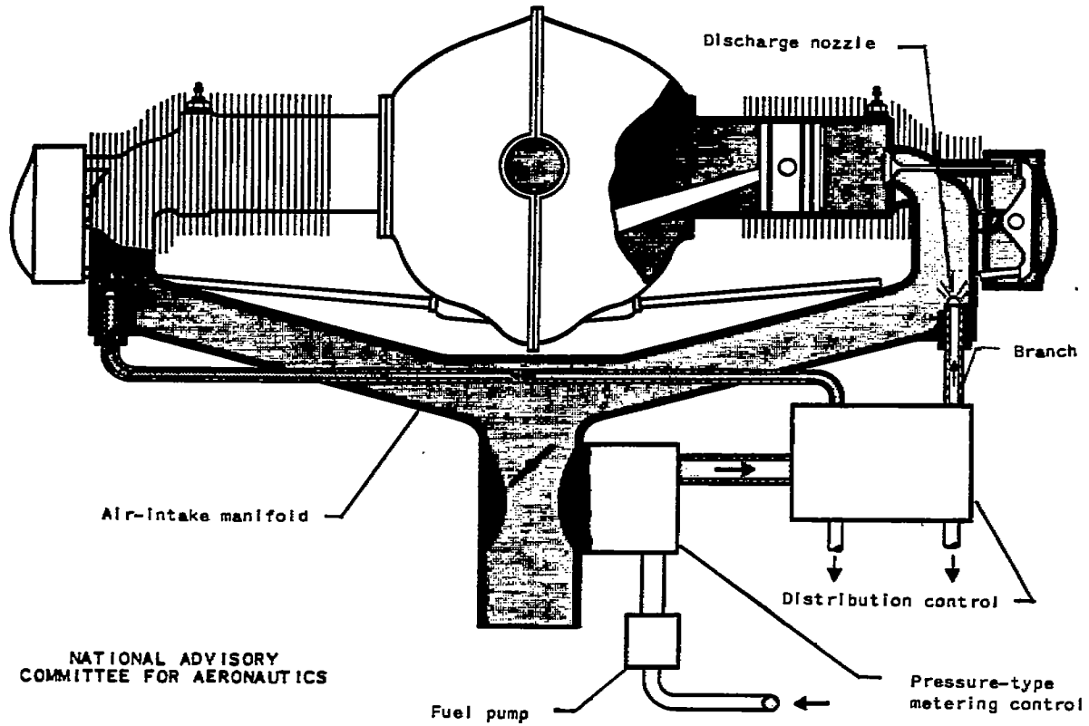
Figure 7. - Schematic diagram showing suggested method of installation of fuel-distribution control on reciprocating engine.
