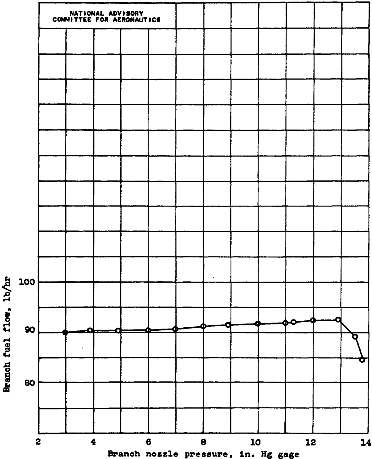
Figure 10. - Effect of varying discharge-nozzle pressure on branch fuel flow of experimental model of fuel-distribution control. Three discharge nozzles held at 11.3 inches of mercury gage; total fuel flow, 370 pounds per hour.
