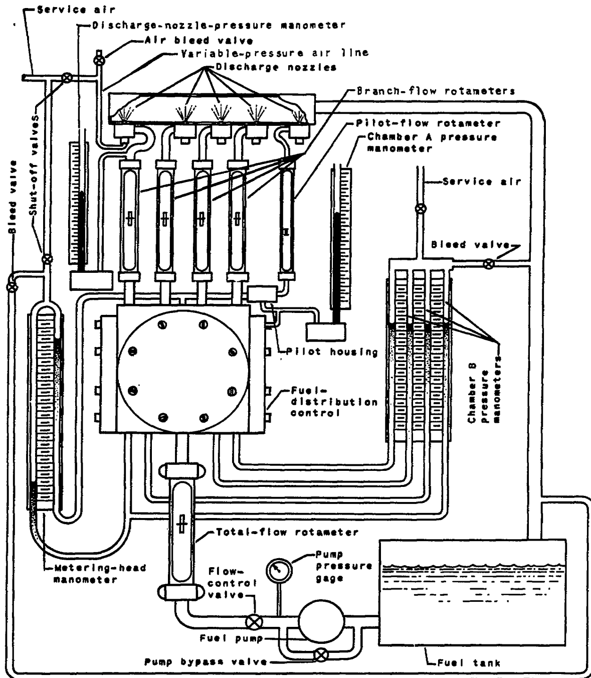
Figure 5. - Schematic diagram of apparatus with experimental model of fuel-distribution control.
