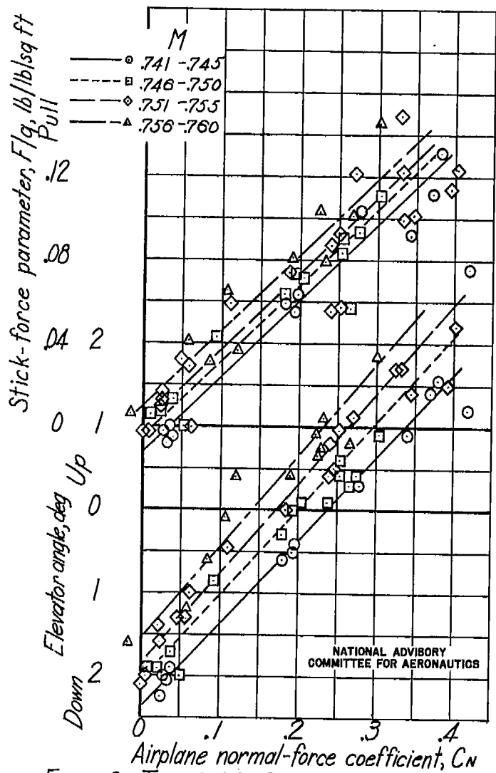
Figure 8.- Typical data from which resultant curves were obtained.
