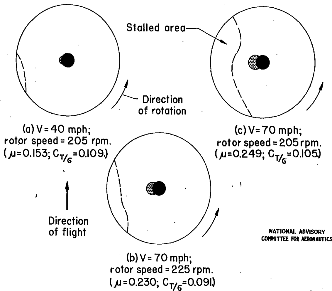
Figure 1.- Theoretical stall boundaries for representative helicopter conditions. Weight, 2580 pounds; radius, 19 feet; parasite-drag area, 23 square feet; stalling angle of attack, 12^\circ .
