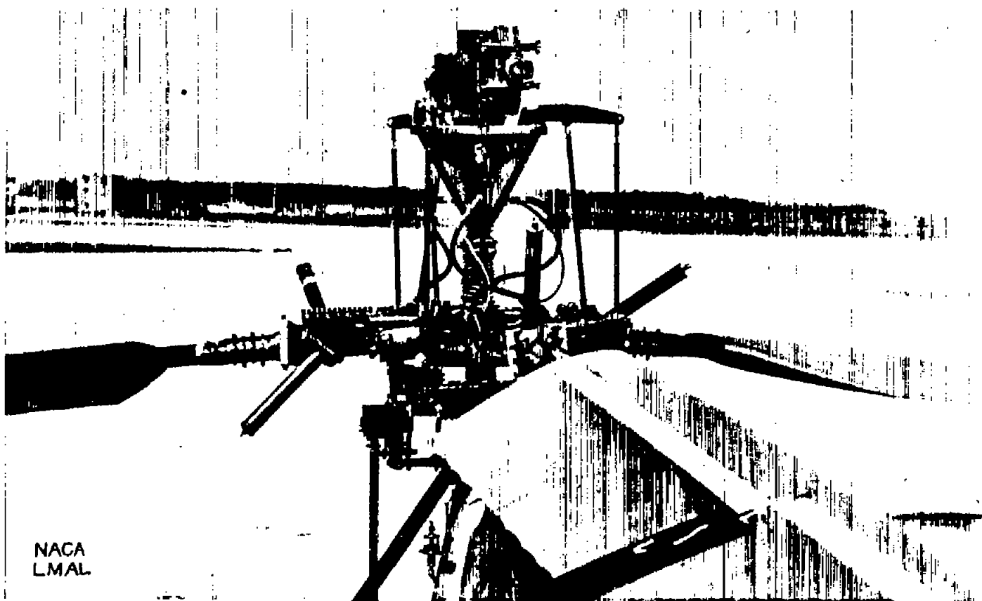
Figure 2.- Camera installation on helicopter rotor hub.
