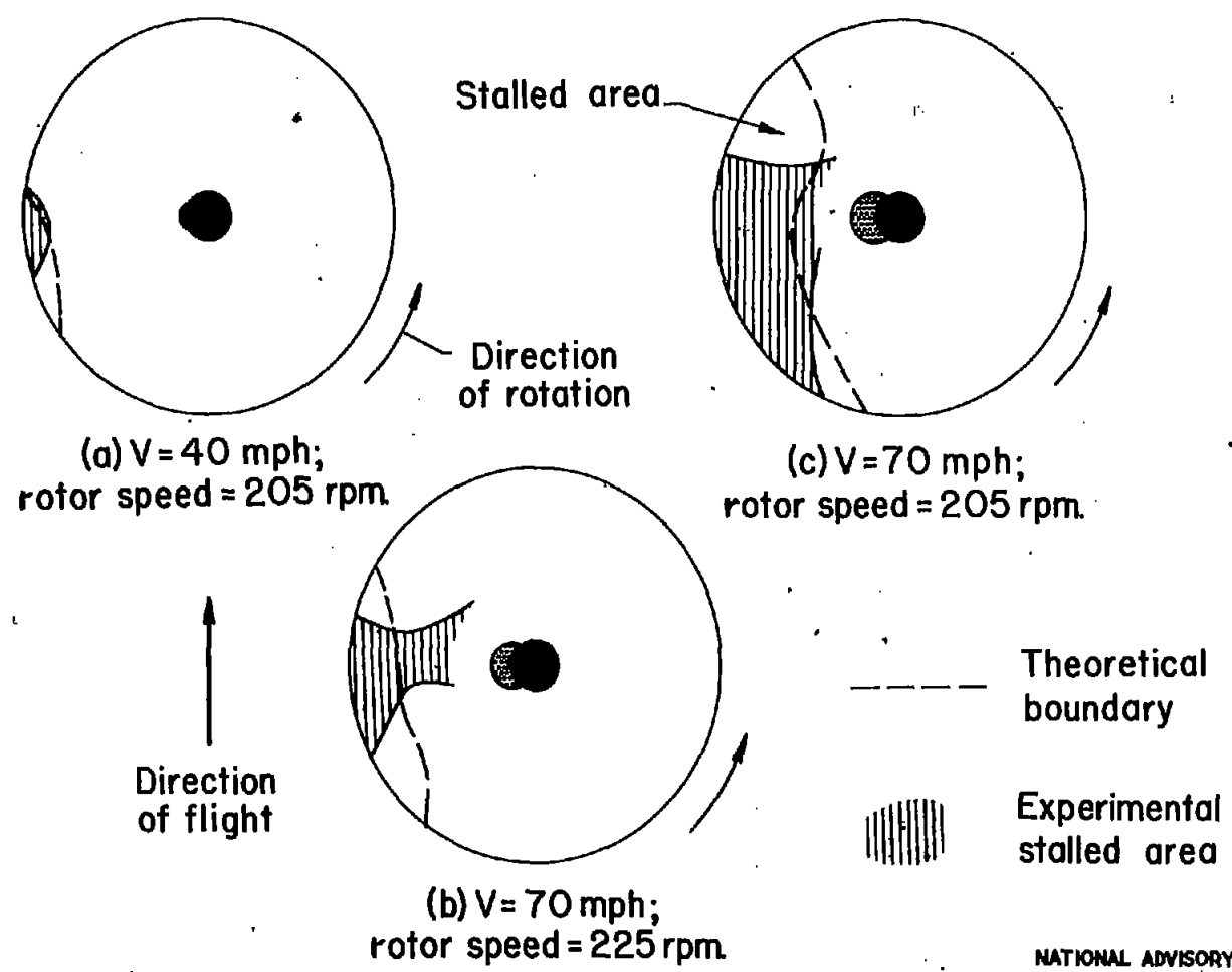
Figure 4.- Comparison between theoretical and experimental stalled areas.
