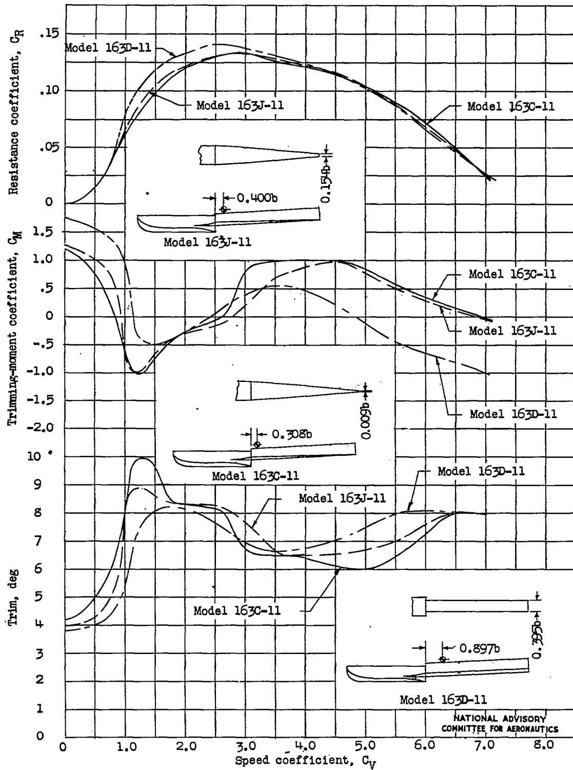
Figure 12.- Effect on best-trim characteristics of tapering afterbody.
