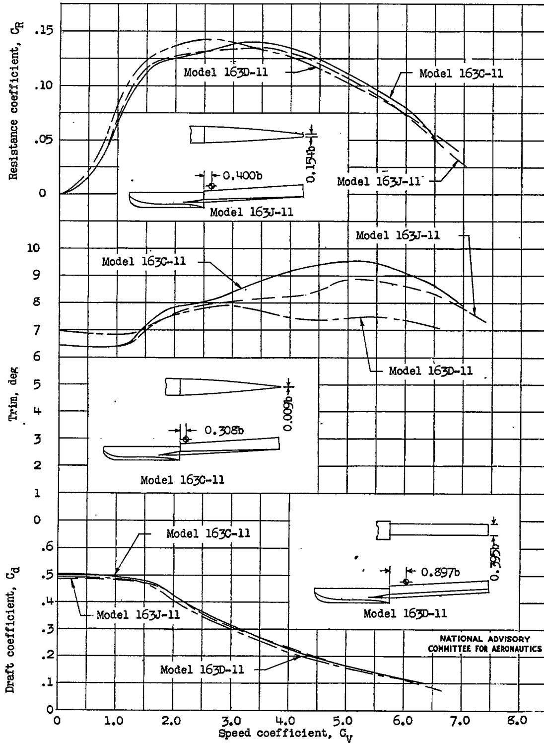
Figure 13.- Effect on free-to-trim characteristics of tapering afterbody.
