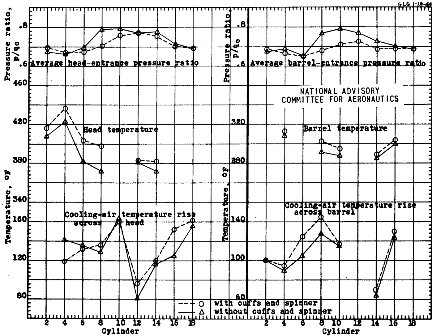
Figure 8. - Pressure and temperature distribution for front cylinders with and without propeller cuffs and spinner. Indicated airspeed, 200 miles per hour; engine speed, 2600 rpm; 1000 brake horsepower; cowl flaps closed. Cylinder temperatures with cuffs and spinner corrected to flight conditions without cuffs and spinner.
