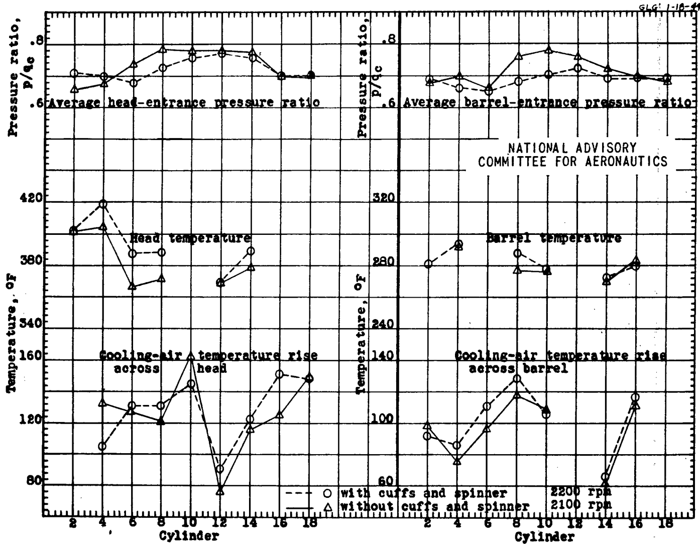
Figure 6. - Pressure and temperature distribution for front cylinders with and without propeller cuffs and spinner. Indicated airspeed, 200 miles per hour; 1000 brake horsepower; cowl flaps closed. Cylinder temperatures with cuffs and spinner corrected to flight conditions without cuffs and spinner.
