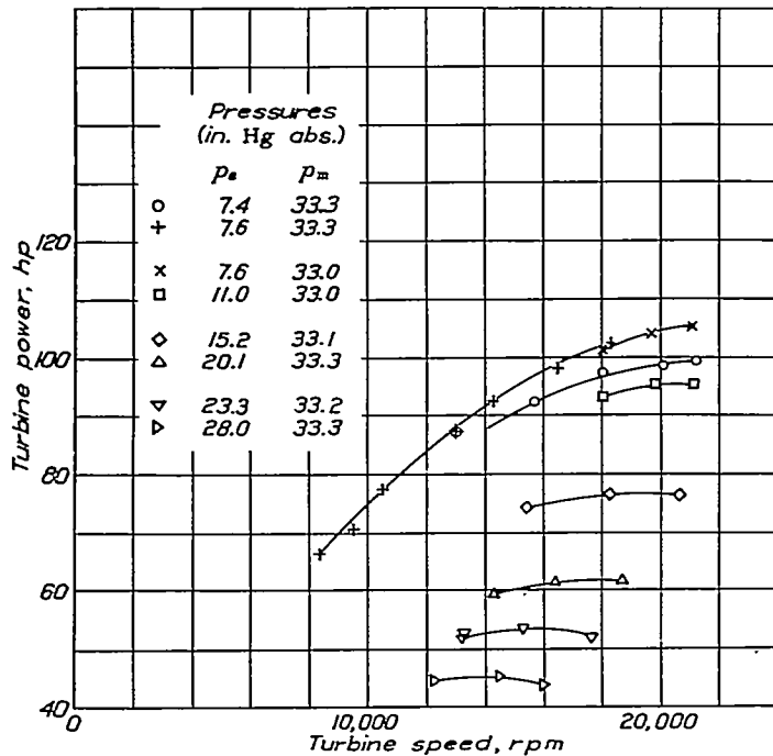
FIGURE 5.—Variation of turbine power with turbine speed. Engine speed, 2000 rpm; full throttle.
