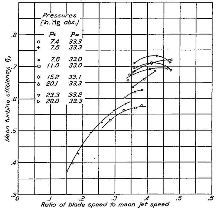
FIGURE 6.—Variation of mean turbine efficiency with ratio of blade speed to mean jet speed. Engine speed, 2000 rpm; full throttle.
