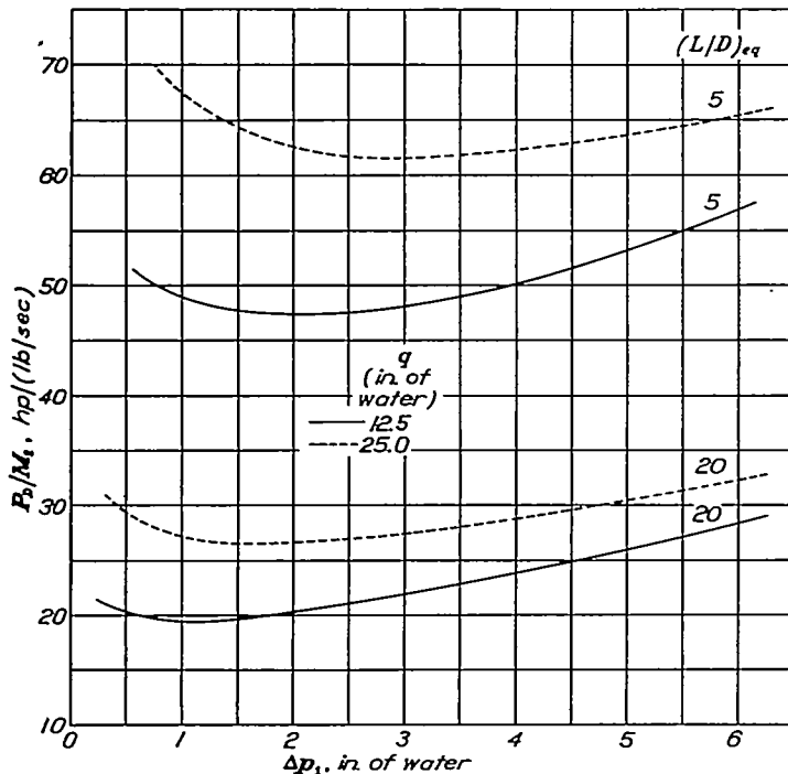
FIGURE 2.—Variation of plate-intercooler drag loss with cooling-air pressure drop for optimum cooling-air flow when (L/D)_{eq} is 5 and 20, and q is 12.5 and 25 inches of water. Altitude, 50,000 feet; \eta , 85 percent.
