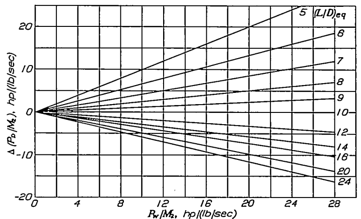
FIGURE 8.—Variation of intercooler drag loss with (L/D)_{eq} .
