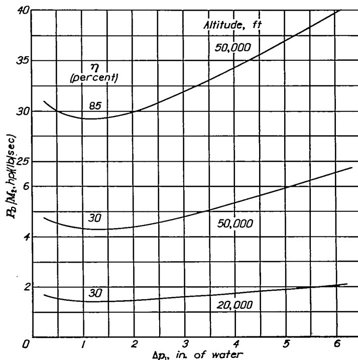
FIGURE 1.—Variation of plate-intercooler drag loss with cooling-air pressure drop for optimum cooling-air flow. (L/D)_{eq} 10; q , 12.5 inches of water; \sigma_{a,r,2} \Delta p_{f,2} 6 inches of water.
