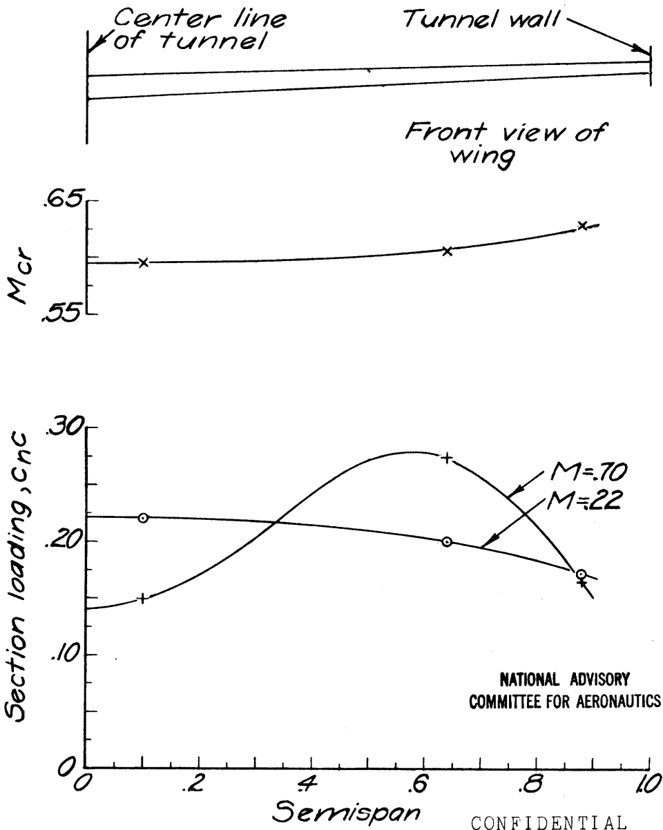
Figure 2.- Measured spanwise load distributions and spanwise variation of section critical Mach number on tapered wing with root-section thickness ratio of 22 percent and tip-section thickness ratio of 12 percent at C_L = 0.2 .
