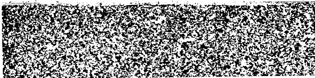
Figure 6. Taper Section of Electrolytically Polished SAE X4130 Fatigue Test Specimen. Horizontal Magnification 100X, Vertical Magnification 1000X. Etched With Nital.
