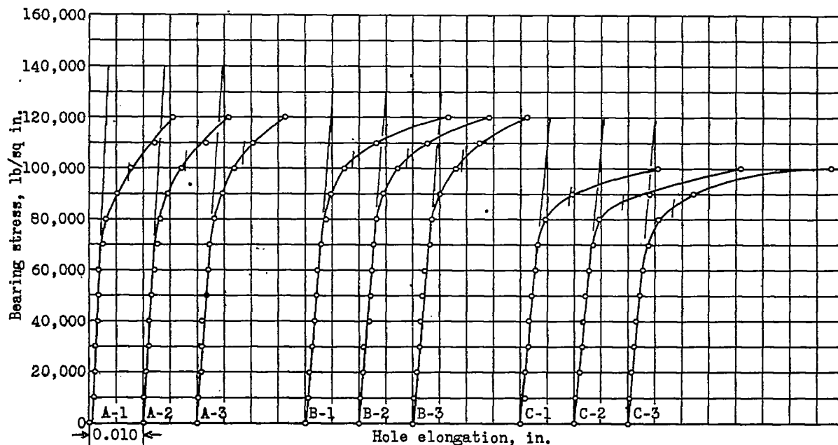
Figure 10.- Bearing stress-hole elongation curves for aluminum alloy sheet, 61S-T.
