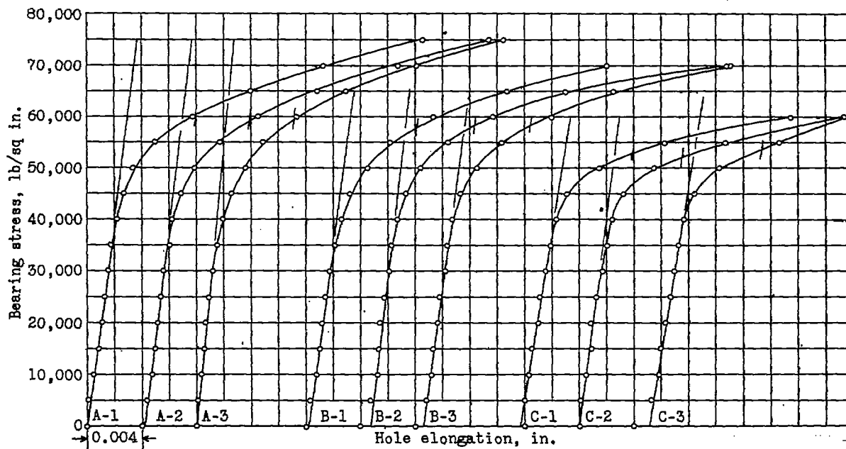
Figure 8.- Bearing stress-hole elongation curves for aluminum alloy sheet, 52S-H.
