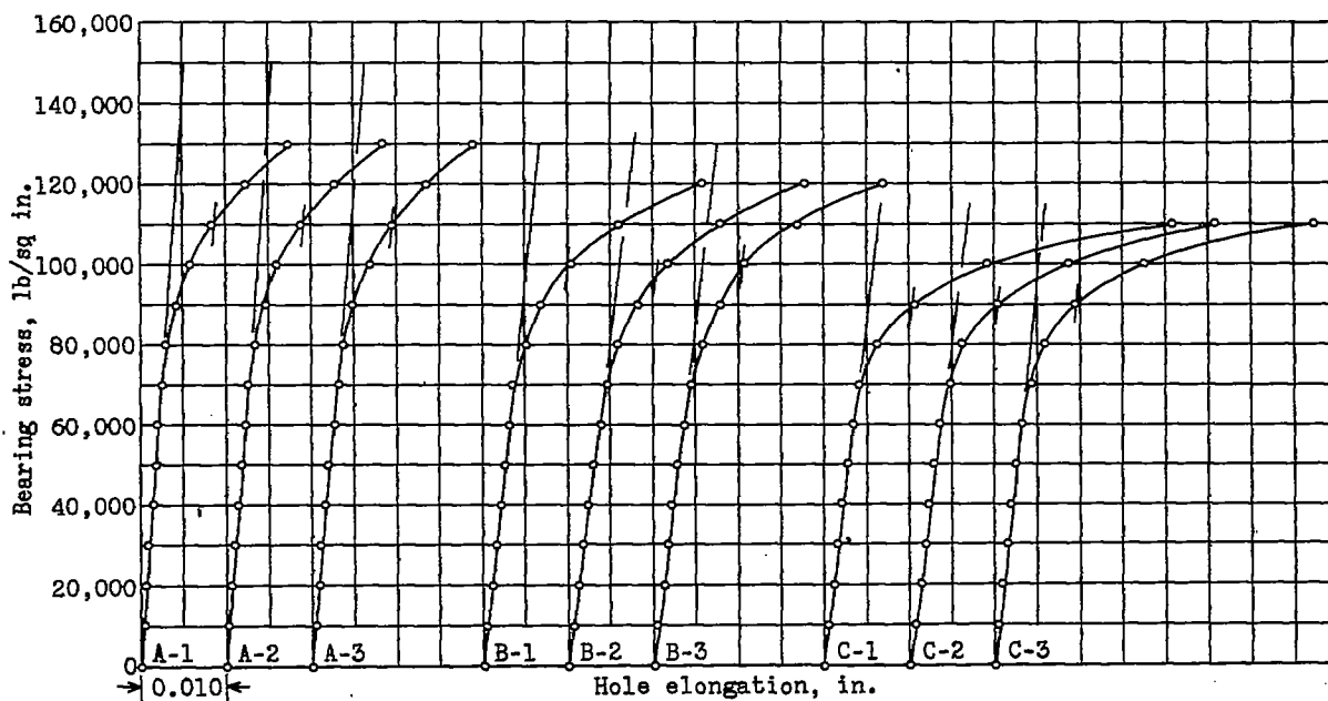
Figure 4.- Bearing stress-hole elongation curves for aluminum alloy sheet, a104d 24S-T.
