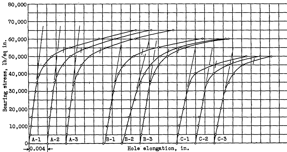
Figure 6.- Bearing stress-hole elongation curves for aluminum alloy sheet, 52S-0.
