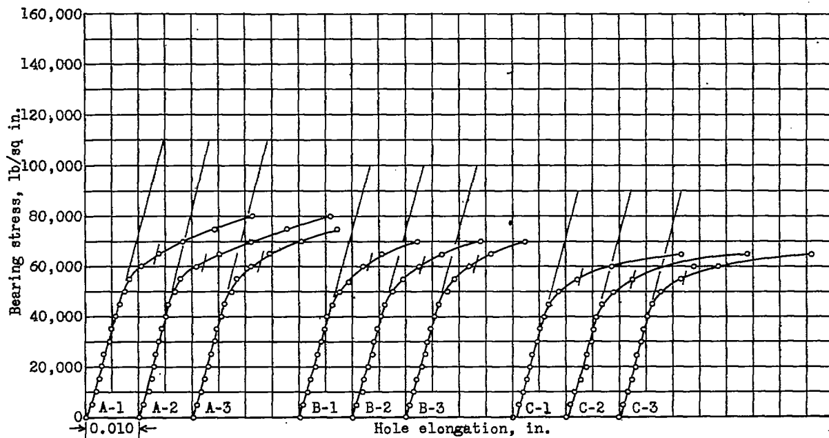
Figure 14.- Bearing stress-hole elongation curves for aluminum alloy extrusion, 53S-T.
