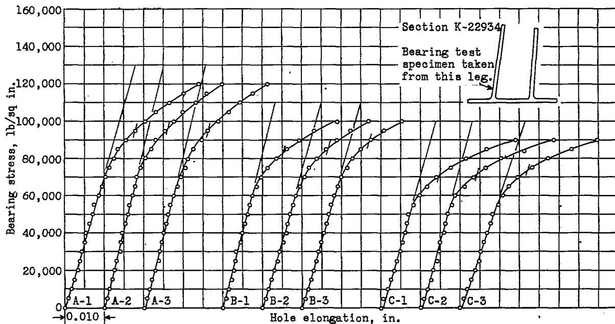
Figure 12.- Bearing stress-hole elongation curves for aluminum alloy forging, A51S-T.
