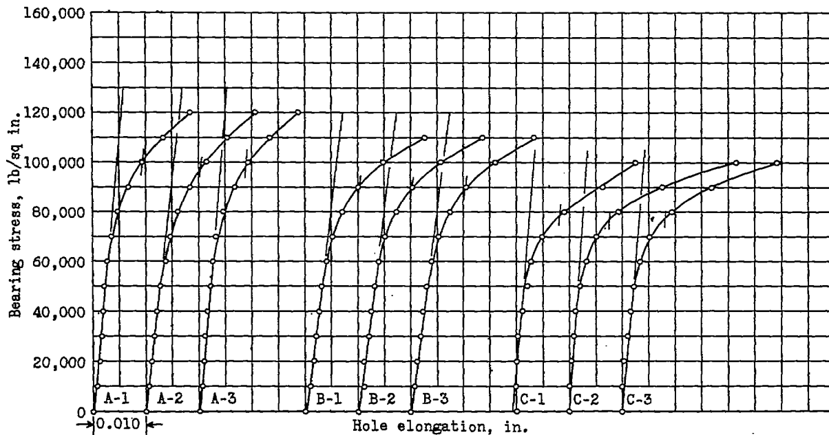
Figure 2.- Bearing stress-hole elongation curves for aluminum alloy sheet, 17S-T.
