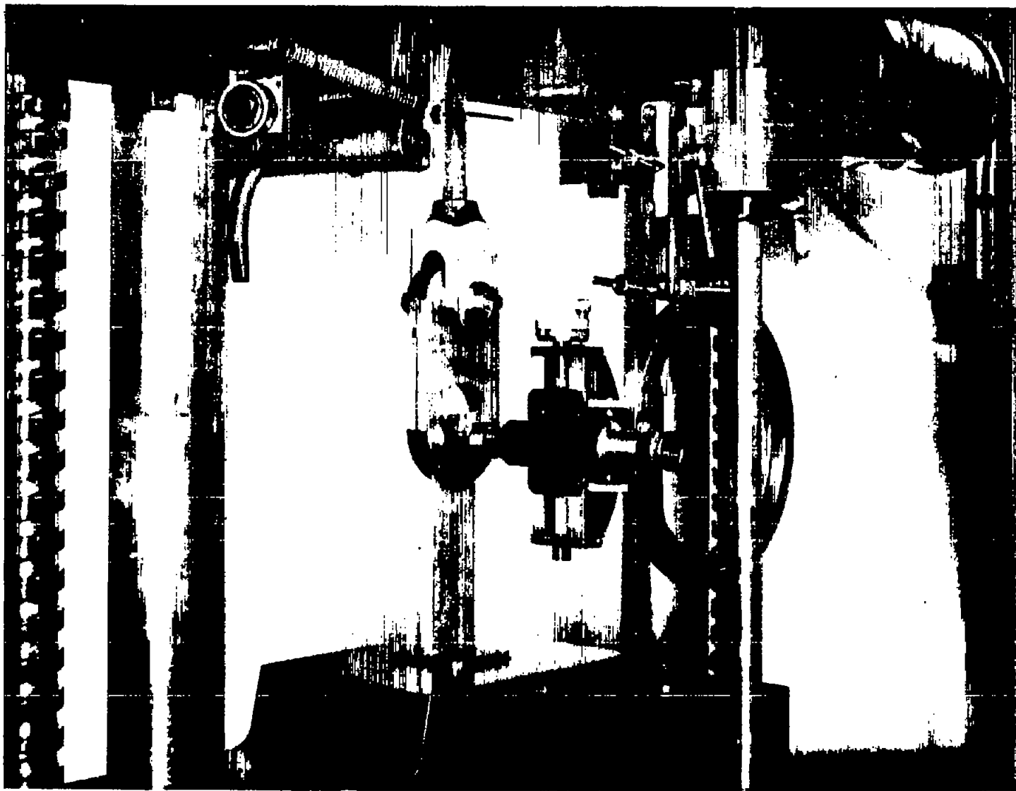
Figure 1.- Arrangement for bearing tests using filar micrometer microscope for measurements of hole elongation.
