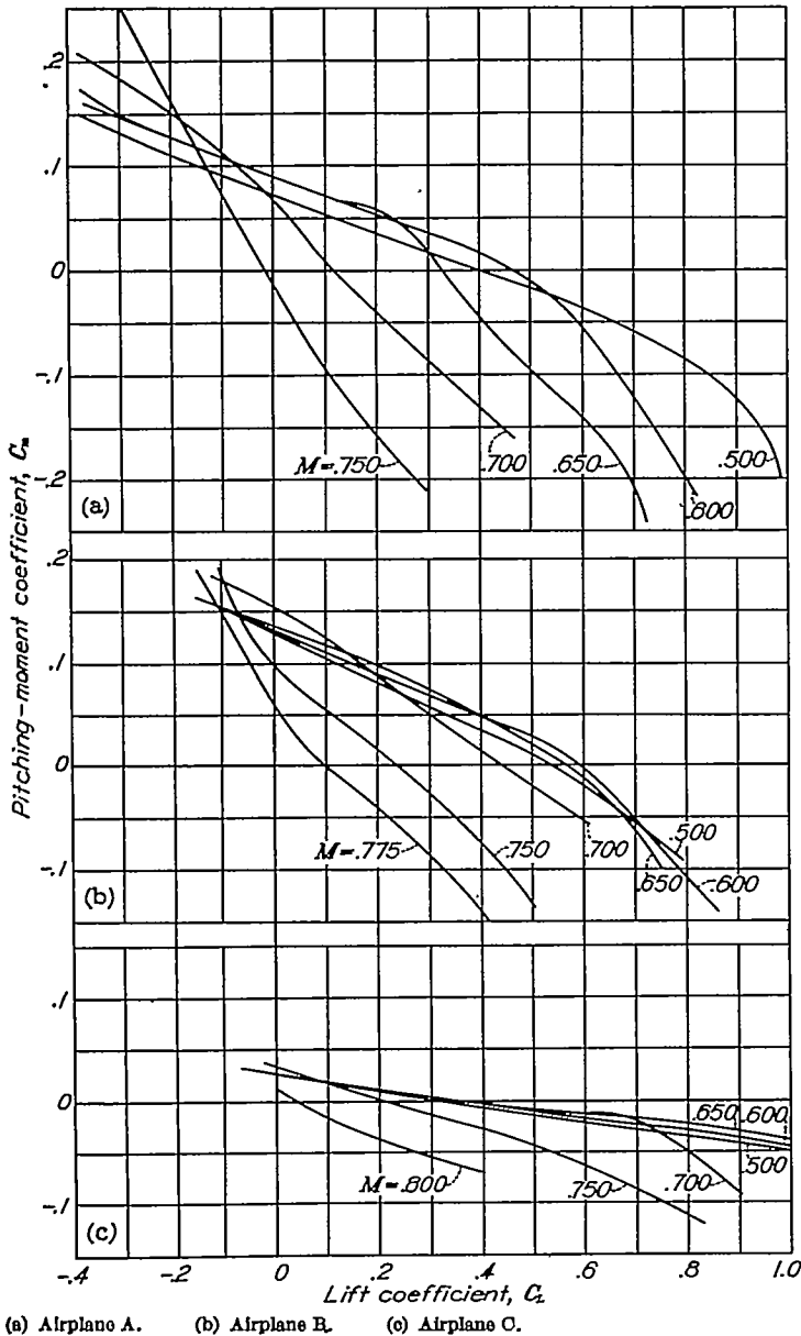
FIGURE 2.—Variation of pitching-moment coefficient with lift coefficient, as a function of Mach number, for three airplanes. Elevators set to trim for level flight at 340 mph and 30,000 ft altitude. ( M=0.50 ).
