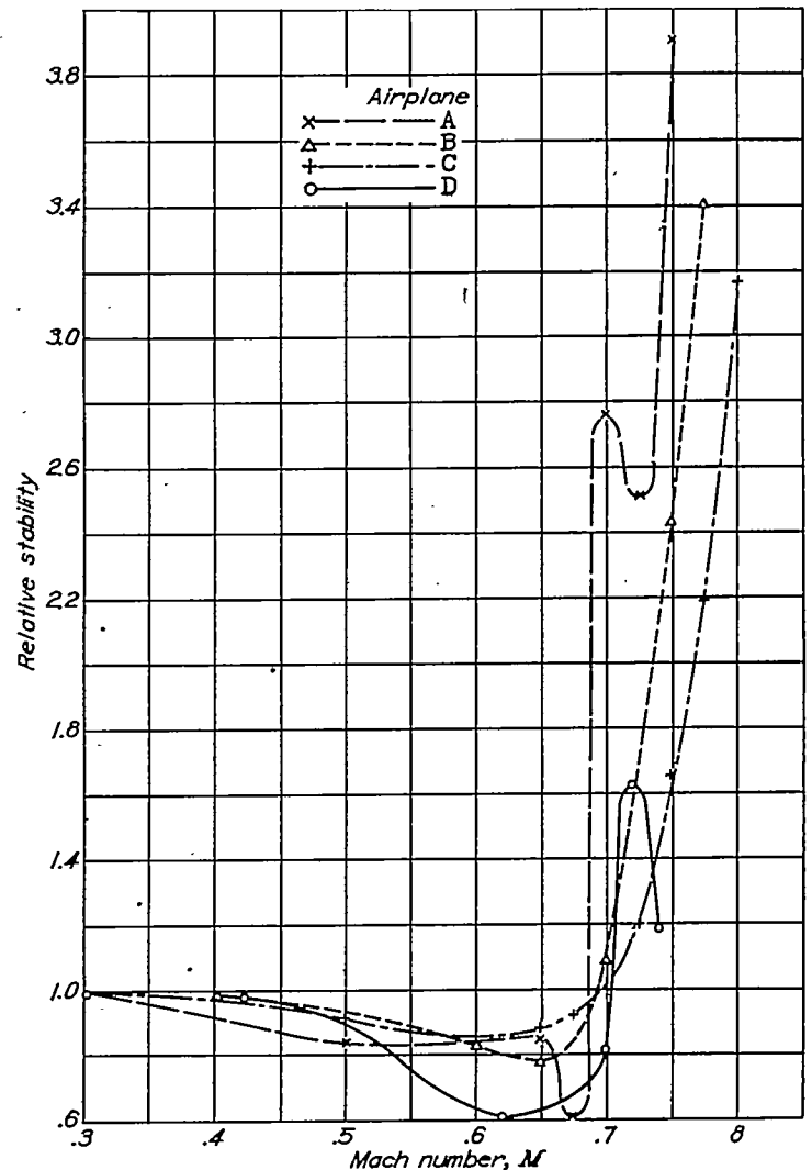
FIGURE 1.—Variation of static longitudinal stability with Mach number for four airplanes at zero lift coefficient. Relative stability = \frac{dC_m/dC_L \text{ at } M}{dC_m/dC_L \text{ at low } M} .
