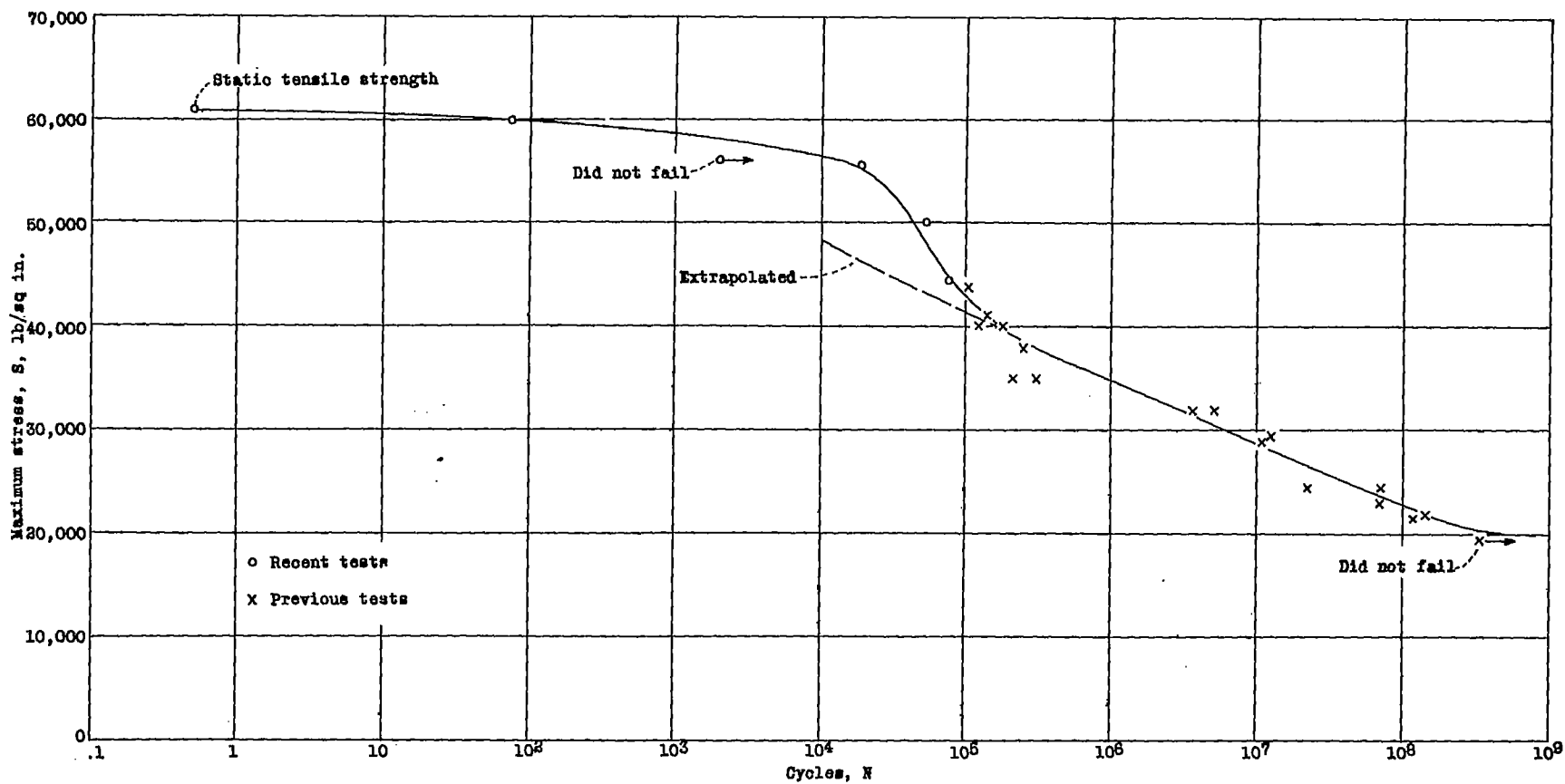
Figure 4.- Direct-stress fatigue curve for 178-T aluminum-alloy rod. Nominal ratio of minimum to maximum stress is equal to zero.
