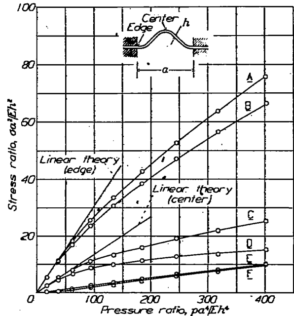
FIGURE 5.—Stresses perpendicular to edge at its midpoint and at the center of a clamped square plate in any direction. \mu , 0.316; \sigma''a^2/Eh^2 , extreme-fiber bending stress ratio; \sigma'a^2/Eh^2 , membrane stress ratio; \sigma a^2/Eh^2 , extreme-fiber stress ratio; pa^4/Eh^4 , pressure ratio.
