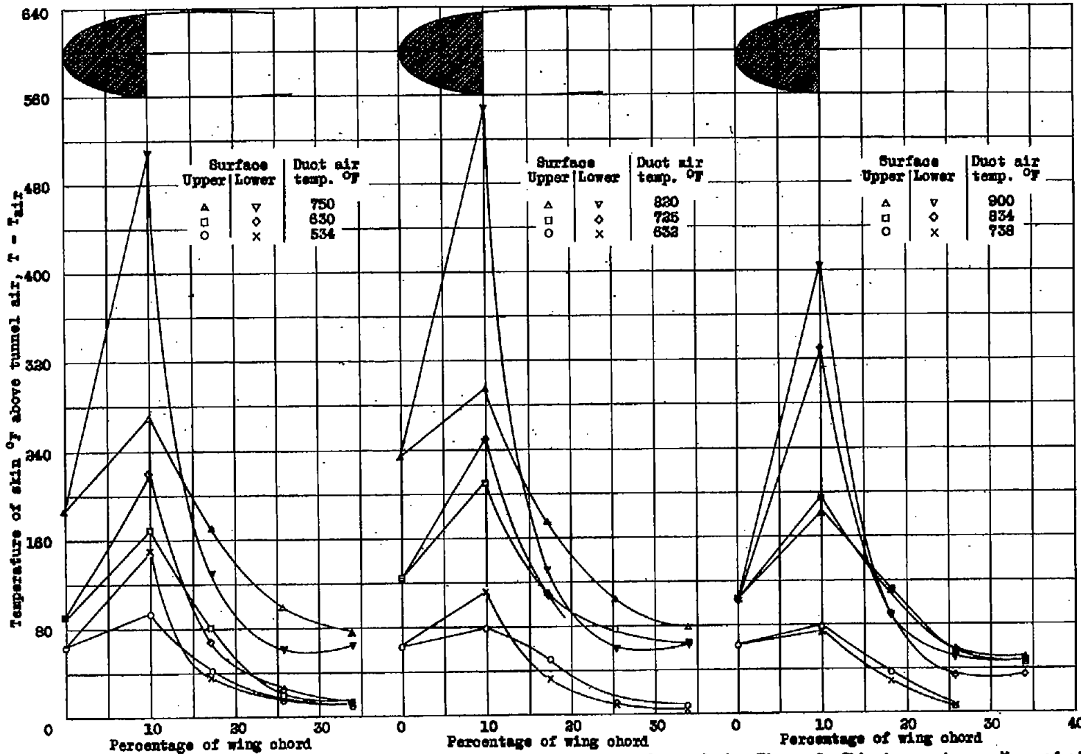
Figure 7.- Skin temperatures. Mass of air through duct = 25.8 lb./min. Model A.
