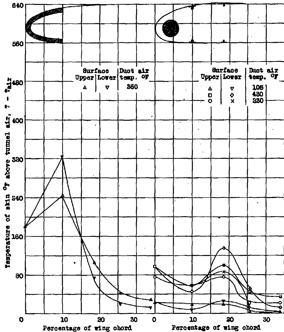
Figure 10.- Skin temperatures. Mass of air through duct = 18 lb./min. Model B.
