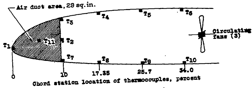
Figure 2.- Model A, heated wing.
