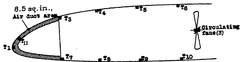
Figure 3.- Model B, heated wing.
