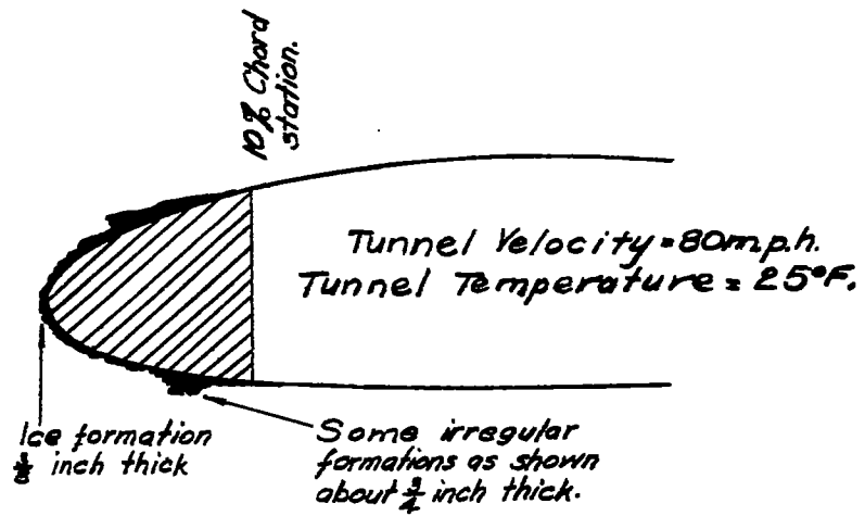
FIGURE 5 Glaze ice on plain wing.
