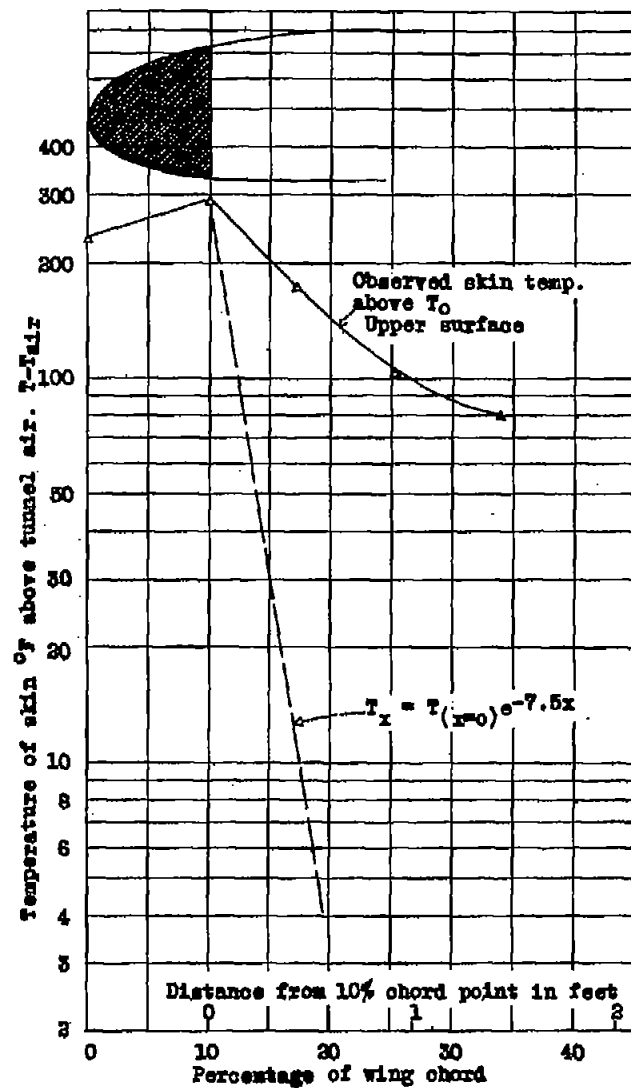
Figure 12.- Skin temperatures. Mass of air through duct = 22.4 lb./min. Model A.
