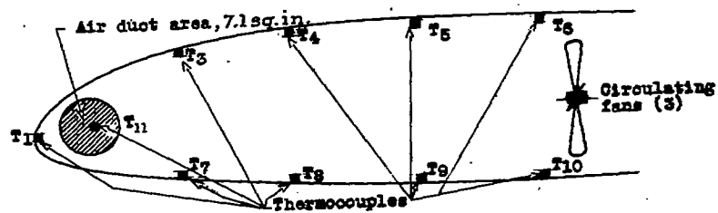
Figure 4.- Model C, heated wing.
