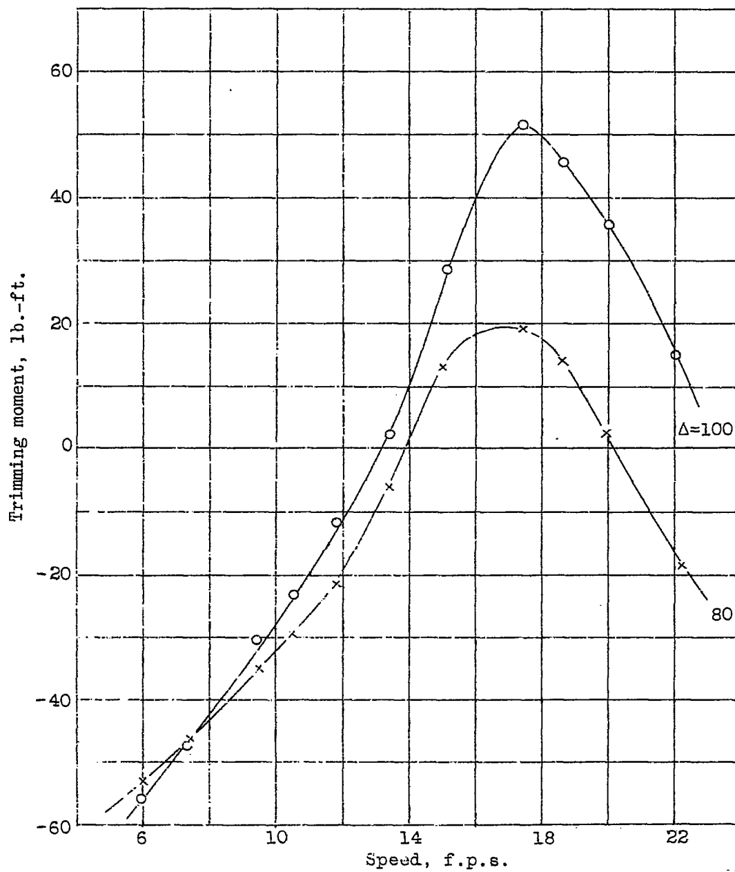
Figure 10.- Model 46. Trimming moment, \tau = 9^\circ (b)
