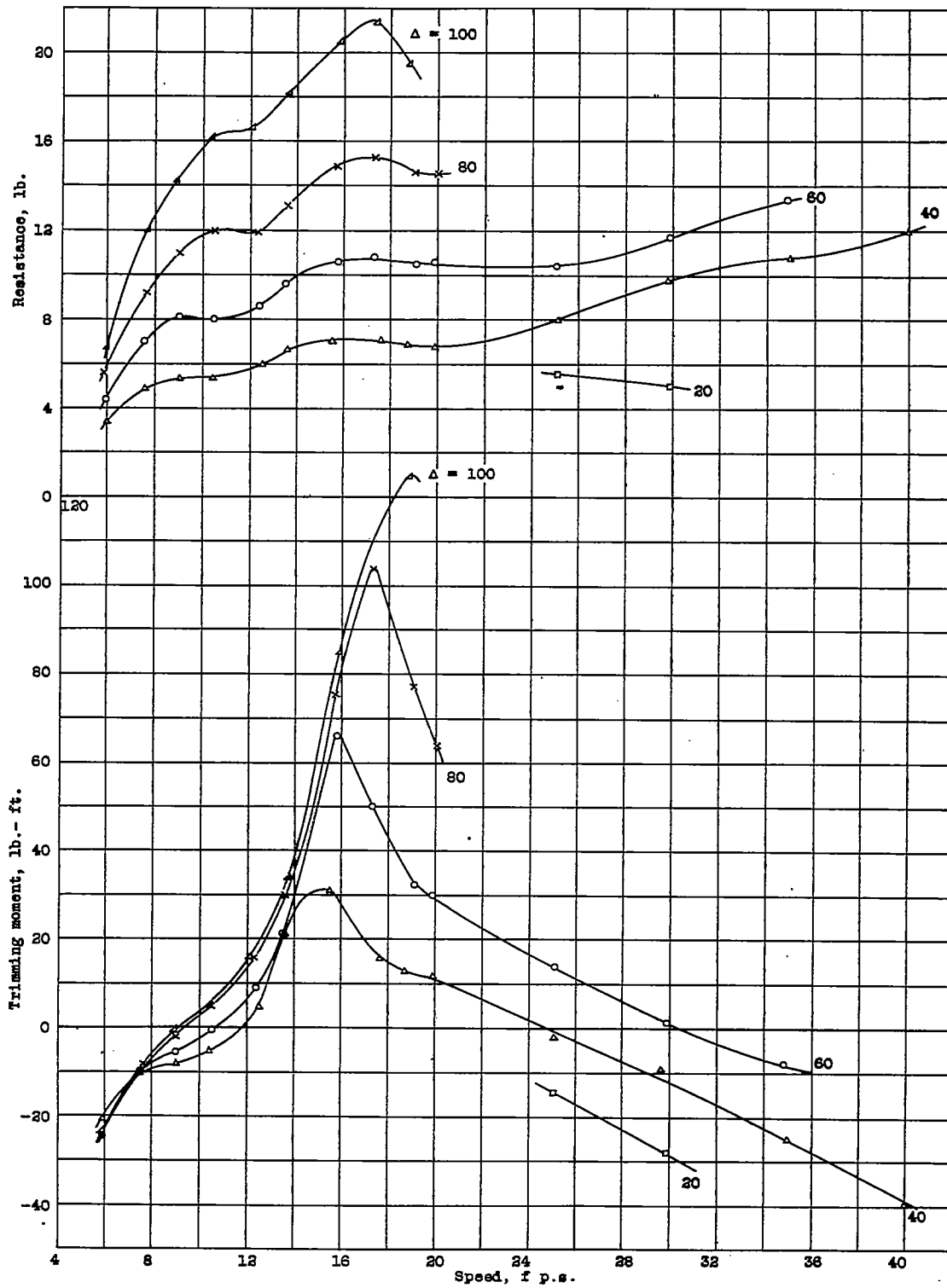
Figure 8. - Model 48. Resistance and trimming moment, \tau = 5^\circ
