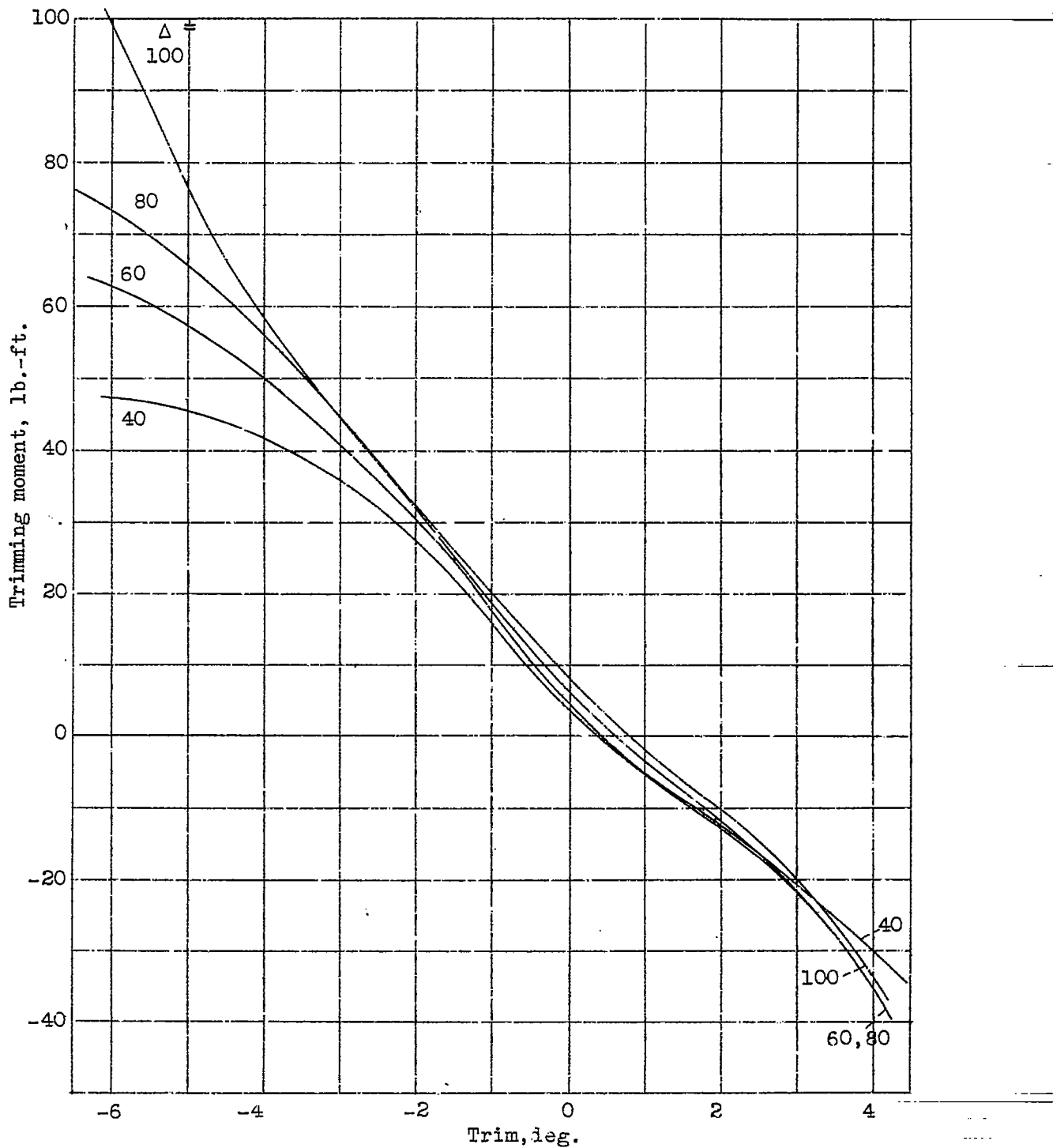
Figure 11.- Model 46. Static trimming moments.
