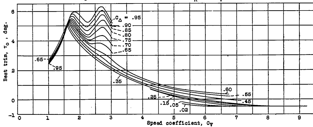
Figure 16. - Model 48. Variation of \tau_0 with C_V .
