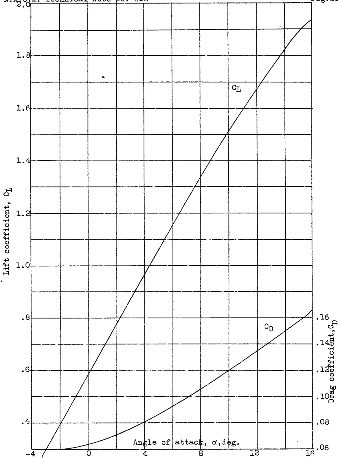
Figure 20.- Lift and drag coefficients of the assumed airfoil with flaps down 30^\circ . Effective aspect ratio, 20.0.
