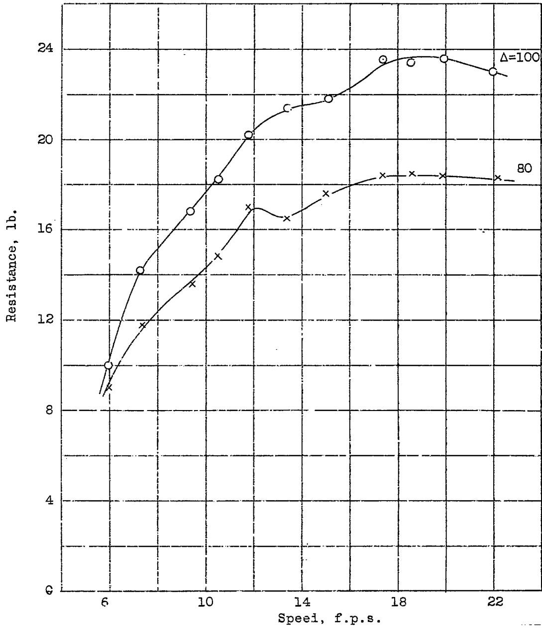
Figure 10.- Model 46. Resistance, \tau = 9^\circ (a)
