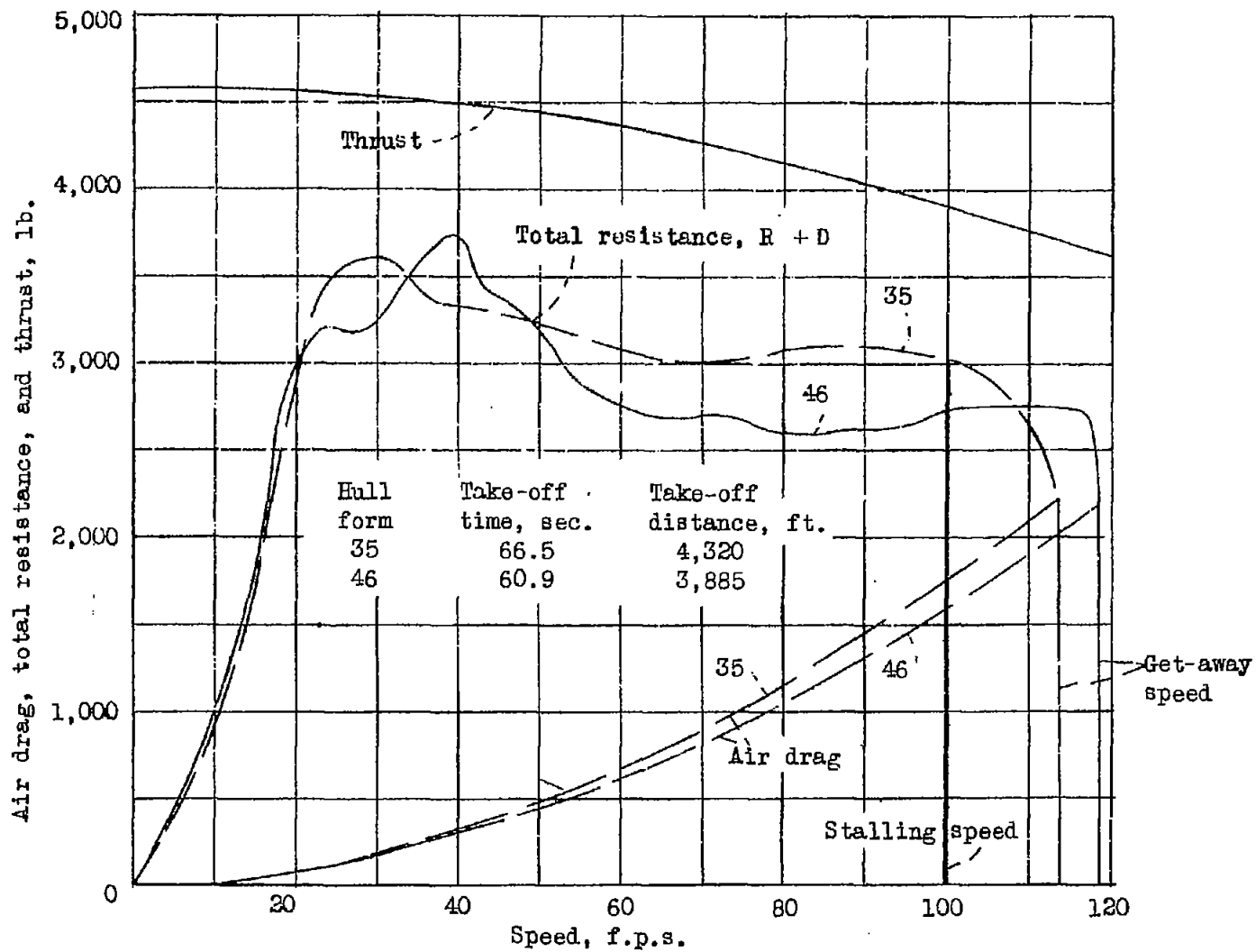
Figure 21. - Take-off comparison of 23,500-lb. flying boats, having twin hulls with the lines of models 35 and 46
