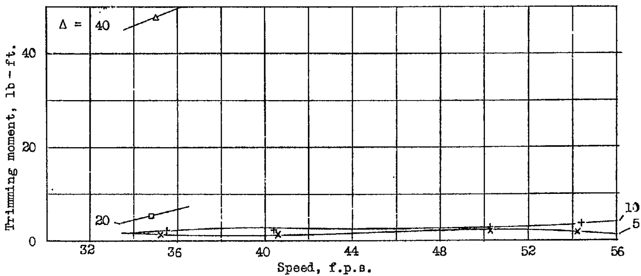
Figure 4. Trimming moment, \tau = -2^\circ Model 46. (b)
