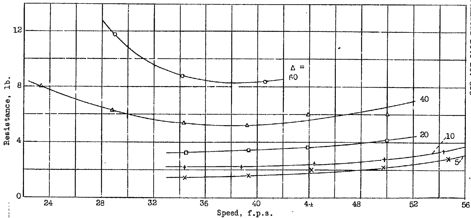
Figure 5. - Model 46. Resistance, \tau = -1^\circ (a)
