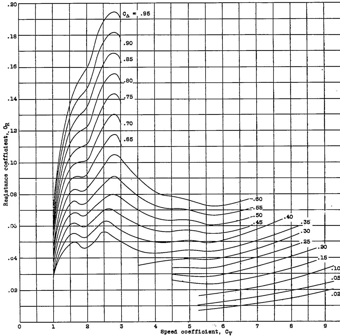
Figure 15. - Model 48. Variation of C_R with C_V at best trim.
