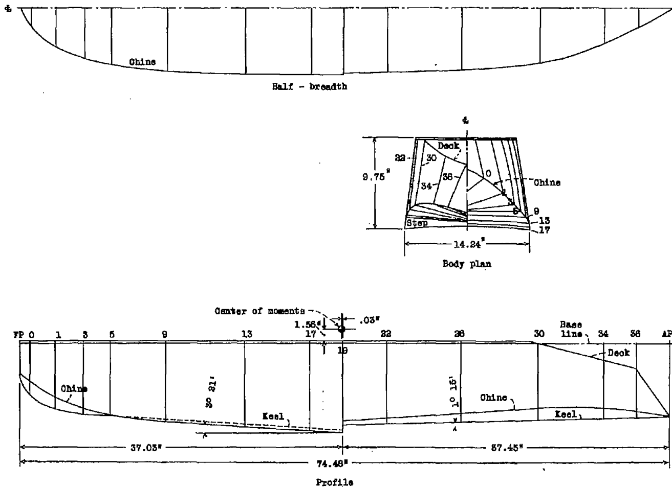
Figure 3. - Lines of N.A.C.A. model 48.
