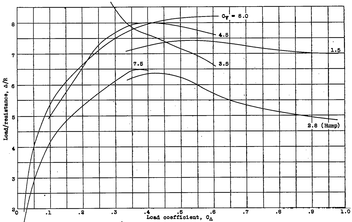
Figure 18.- Model 46. Variation of \frac{\Delta}{R} with C_{\Delta} at best trim.
