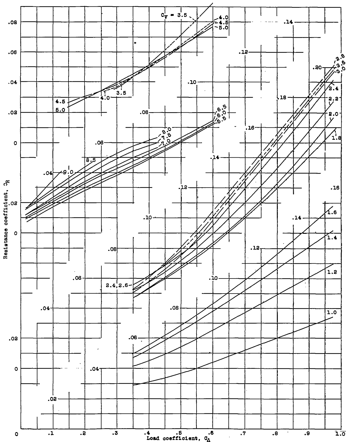
Figure 14. - Model 46. Variation of C_R with C_A at best trim.
