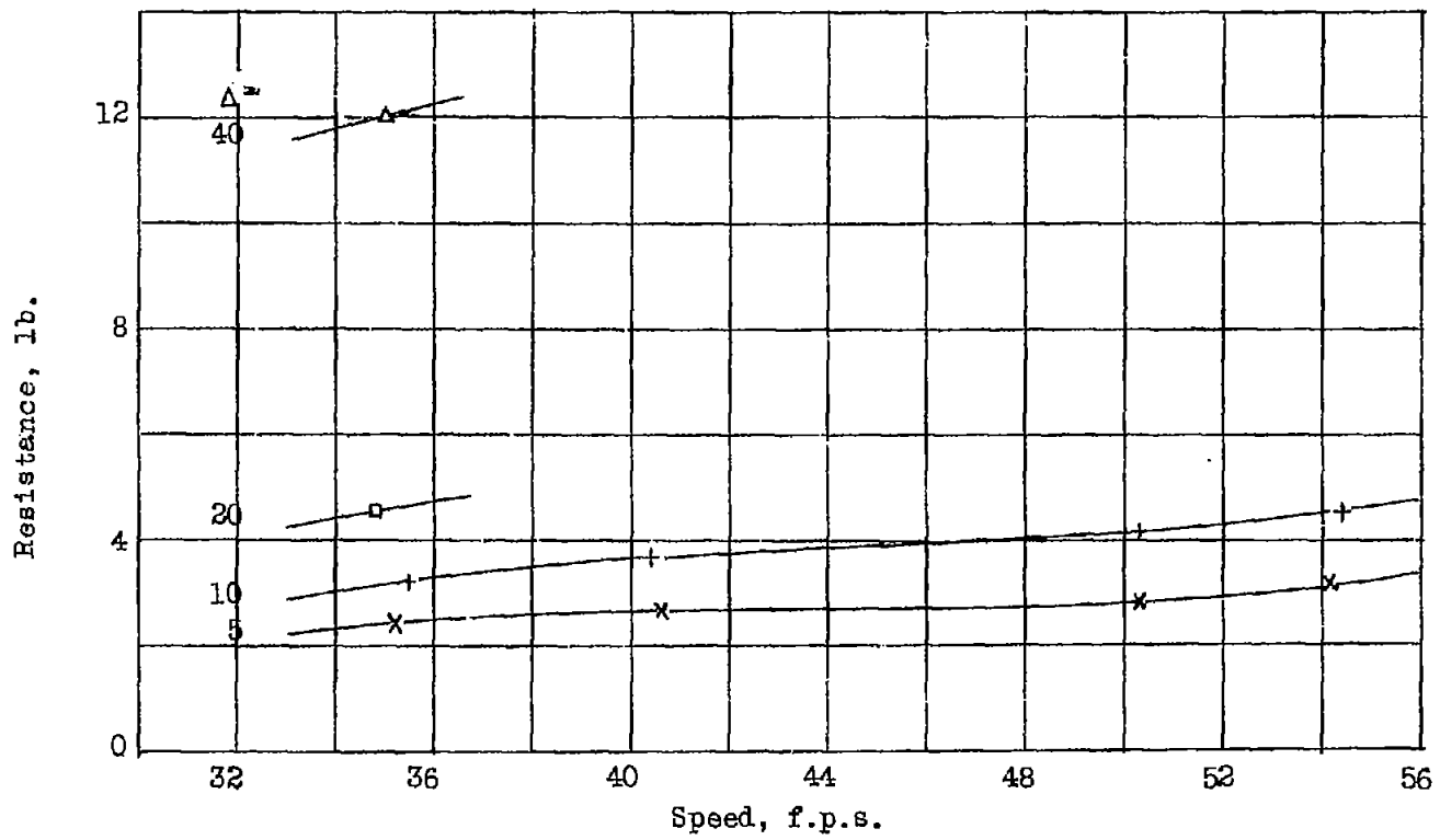
Figure 4. - Model 46. Resistance, \tau = -2^\circ (a)
