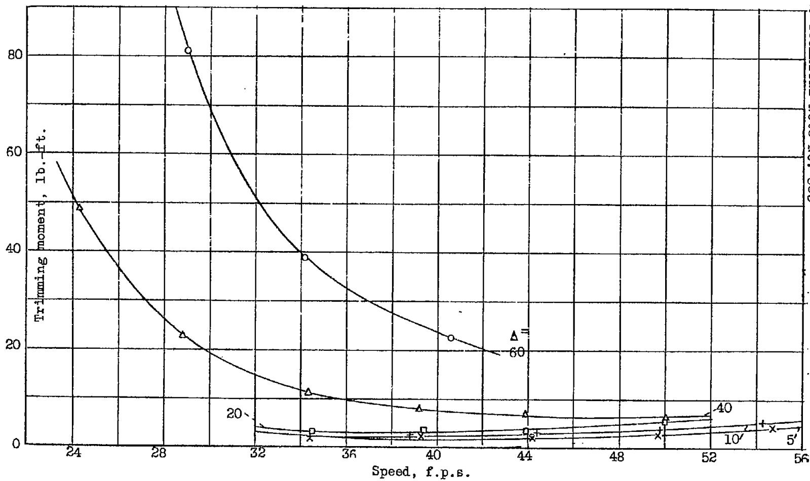
Figure 5. - Model 46. Trimming moment, \tau = -1^\circ (b)
