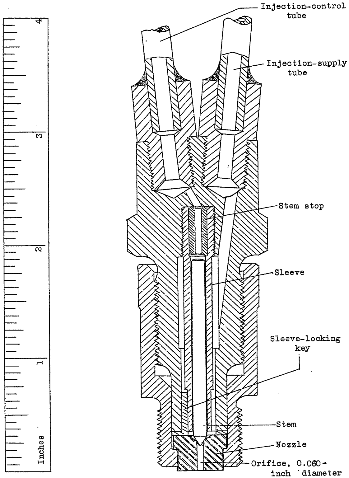
Figure 4.- Fuel-injection-valve assembly
