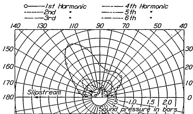
FIGURE 6.—Polar diagram of harmonic distribution.
