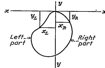
FIGURE 3.—Coordinate system used in the general solution for simple rings.
