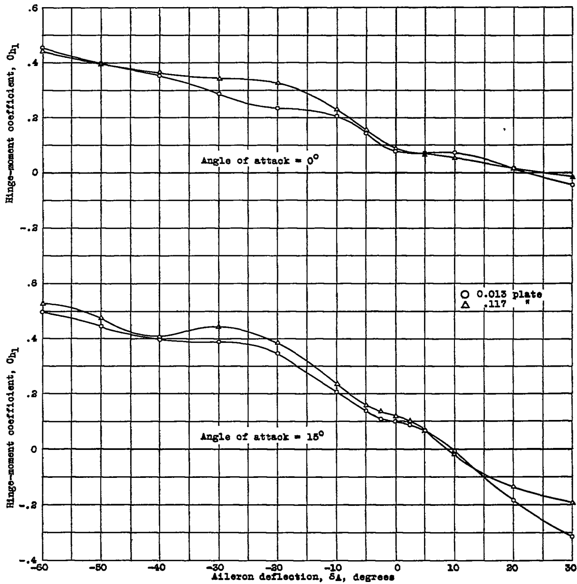
Figure 12.- Hinge-moment coefficients of a slot-lip aileron at 0.30 chord with a slot with a straight front wall with a clearance of 0.13 aileron chord and a slot gap 0.043c and slot width 0.066c.
