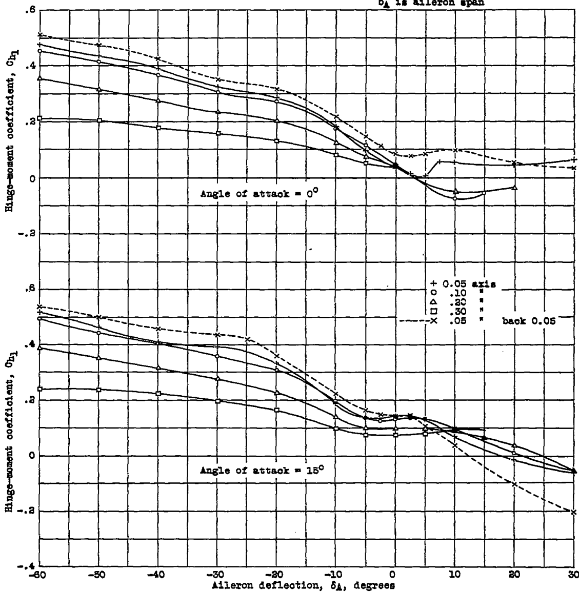
Figure 9.- Hinge-moment coefficients of a slot-lip aileron at 0.30 chord with a special-shape slot of slot gap 0.042c and slot width 0.068c with various aileron hinge-axis positions.
