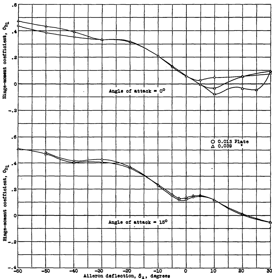
Figure 10.- Hinge-moment coefficients of a slot-lip aileron at 0.30 chord with a slot with a straight front wall with a clearance of 0.028 aileron chord and a slot gap 0.042c and slot width 0.088c.
