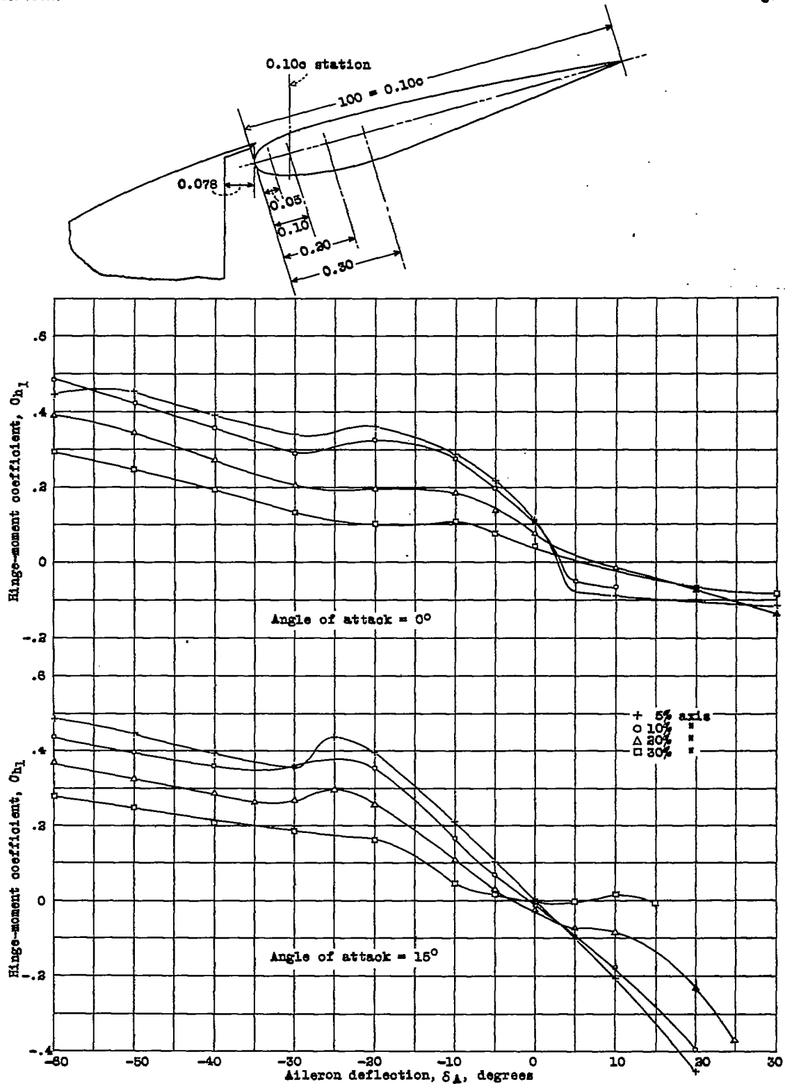
Figure 19.- Hinge-moment coefficients of a slot-lip aileron at 0.10c with 0.078 aileron chord clearance with 0.04c gap and 0.07c width and various aileron-hinge axes.
