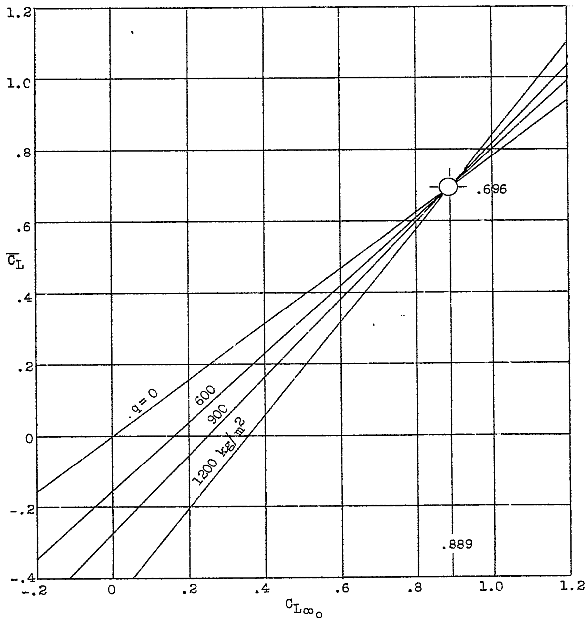
Figure 9.- Variation of \bar{C}_L (absolute lift coefficient of entire wing) with C_{L\alpha_0}
