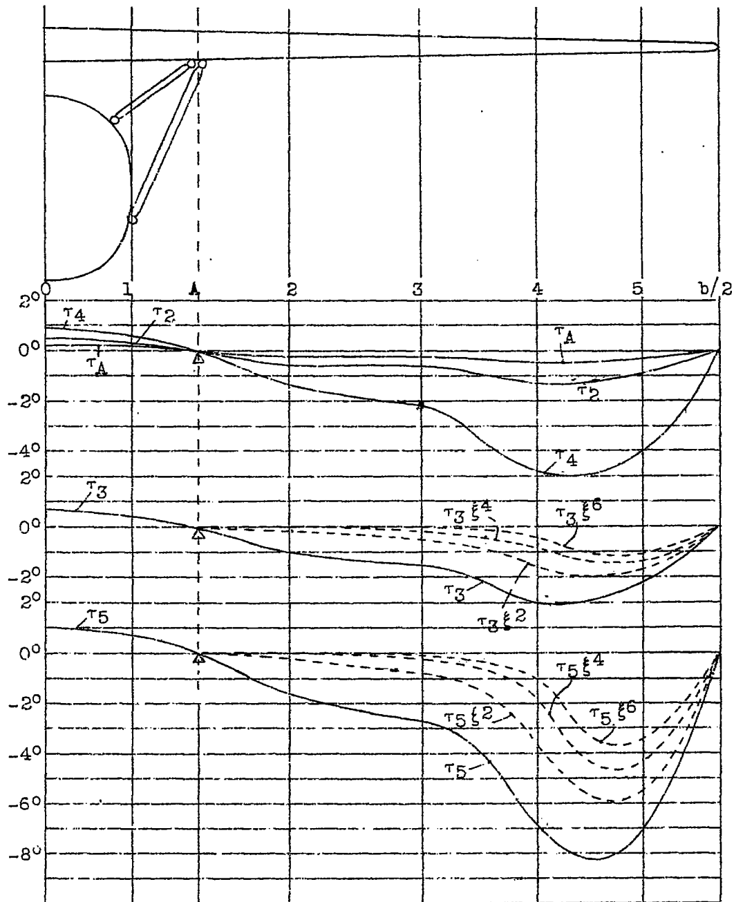
Figure 2.- Lines of influence of the wing twist from D.27 airplane
