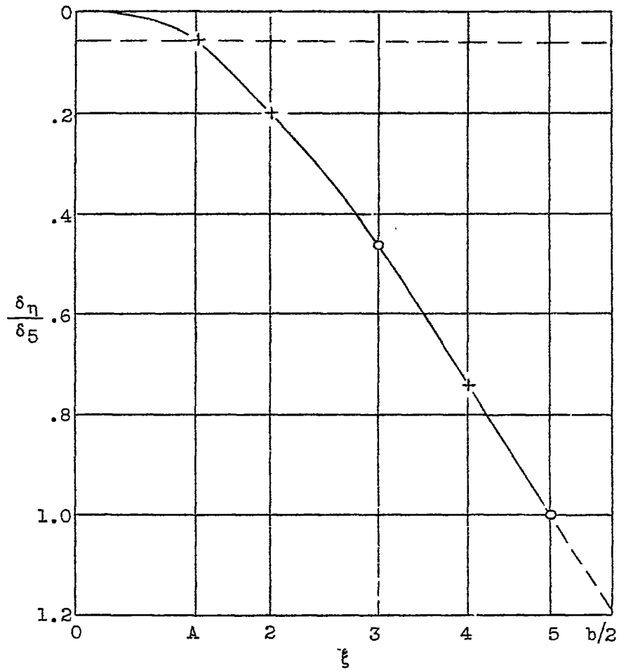
Figure 8.- Variation of \delta \eta / \delta \epsilon with distance from the wing root.
