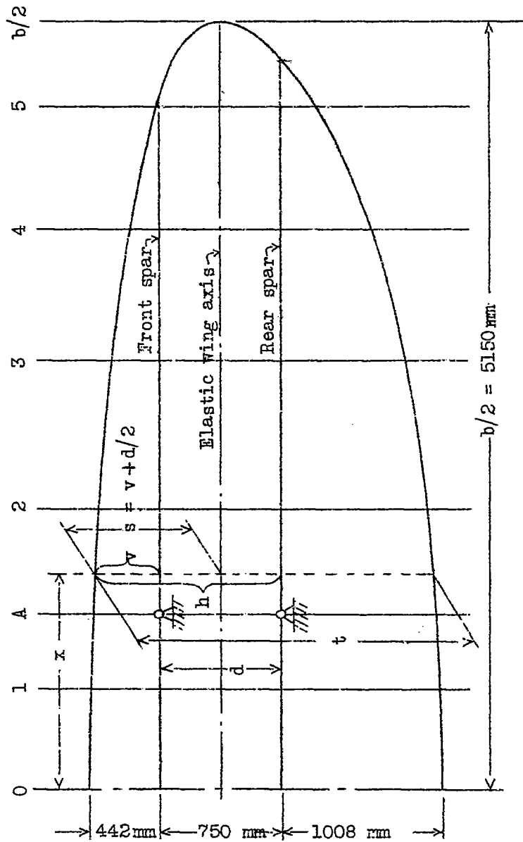
Figure 3.-Elliptical wing with approximately the same area as the standard wing of the D.27 airplane.
