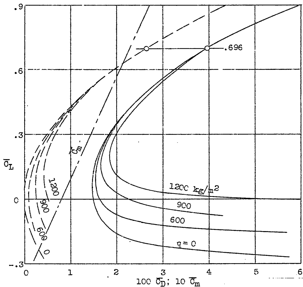
Figure 1C.- Variation of \bar{C}_L (absolute lift coefficient of entire wing) with \bar{C}_D and \bar{C}_m .
