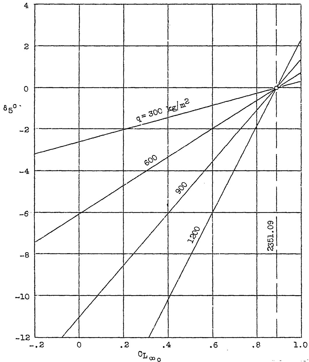
Figure 7.- Variation of \delta_5 with C_{L_{\infty}} and q .
