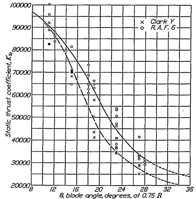
FIGURE 2.—Static thrust coefficients for adjustable blade metal propellers
