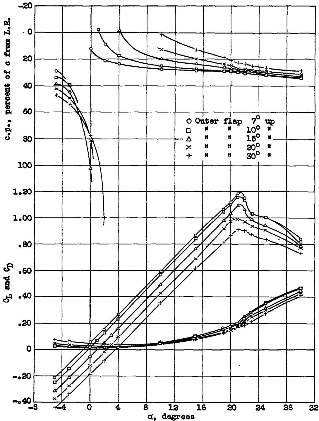
Figure 4.- C_L , C_D and c.p. with full span plain flap divided into four parts of equal span. Center pair set 7° up, outer pair at various angles.
