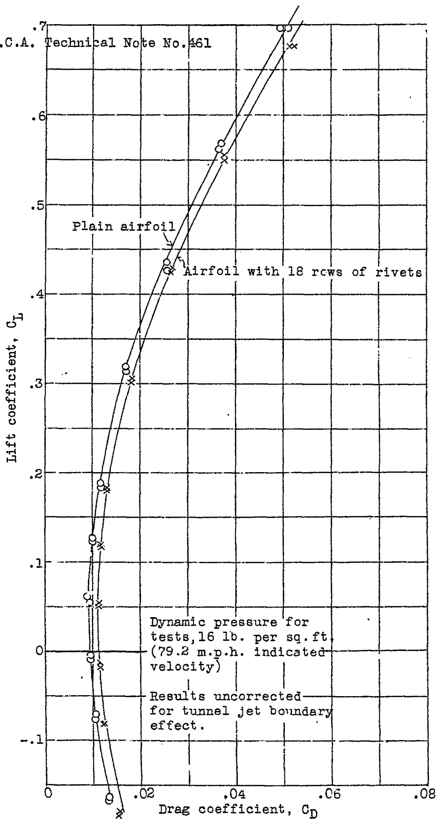
Figure 8.- Polars for plain airfoil and airfoil with rivets.
