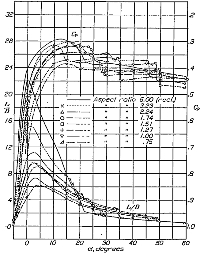
FIGURE 7.—Variations of L/D ratio and center of pressure location with angle of attack, Semicircular tips. 0^\circ yaw
