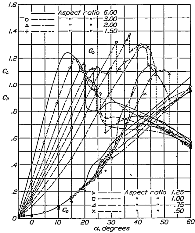
FIGURE 2.—Variations of lift and drag coefficients with angle of attack. Rectangular tips. 0° yaw
