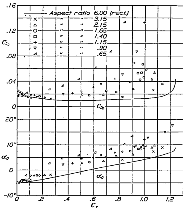
FIGURE 15.—Variations of angle of attack for infinite aspect ratio and profile drag with lift coefficient. Faired tips. 0° yaw
