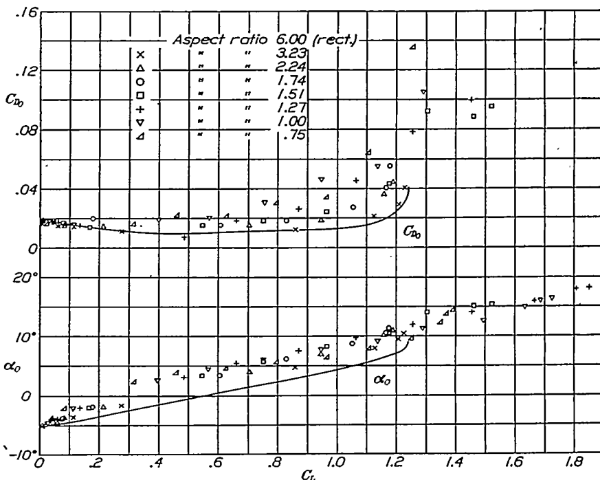
FIGURE 16.—Variations of angle of attack for infinite aspect ratio and profile drag with lift coefficient. Semicircular tips. 0° yaw
