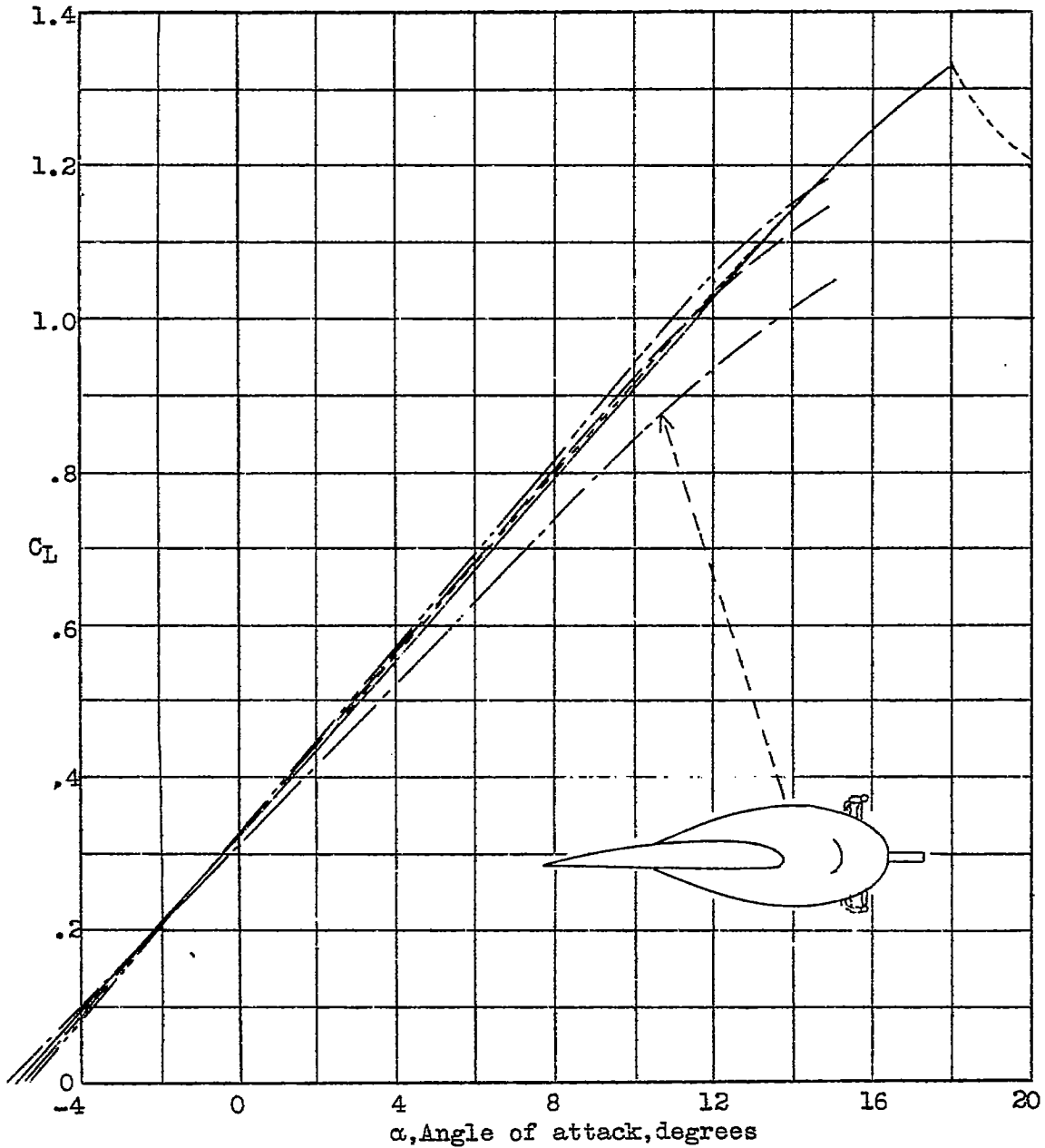
Fig.16 Effect of nacelles on lift coefficient. (Clark Y airfoil, position B).
