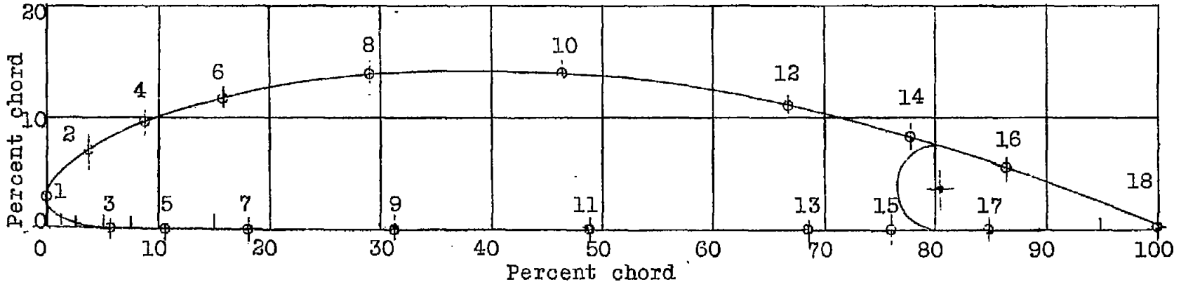
Fig. 2 N.A.C.A. 84M profile showing flap and orifices. 15 in. chord model.
