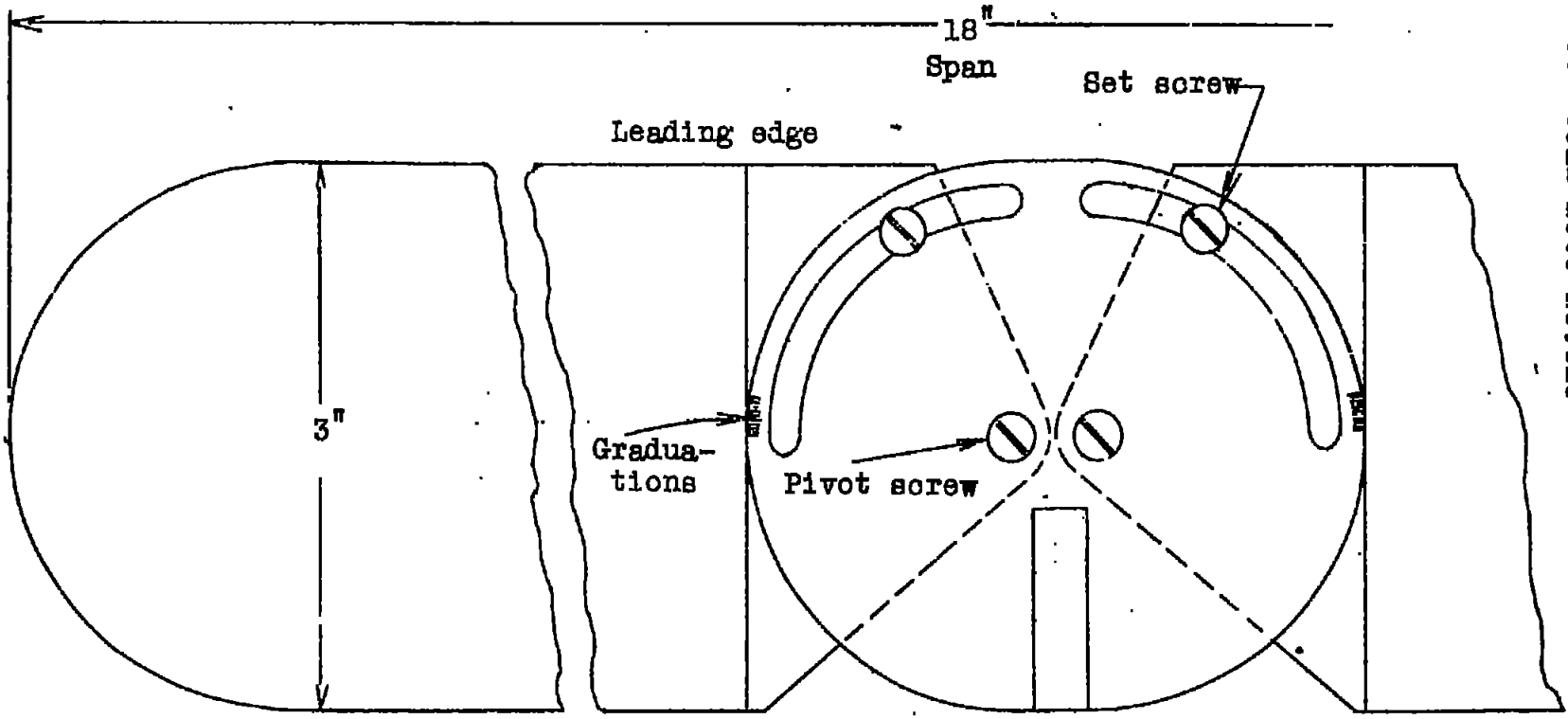
Fig.1 Airfoil with variable sweepback. Clark Y section.
