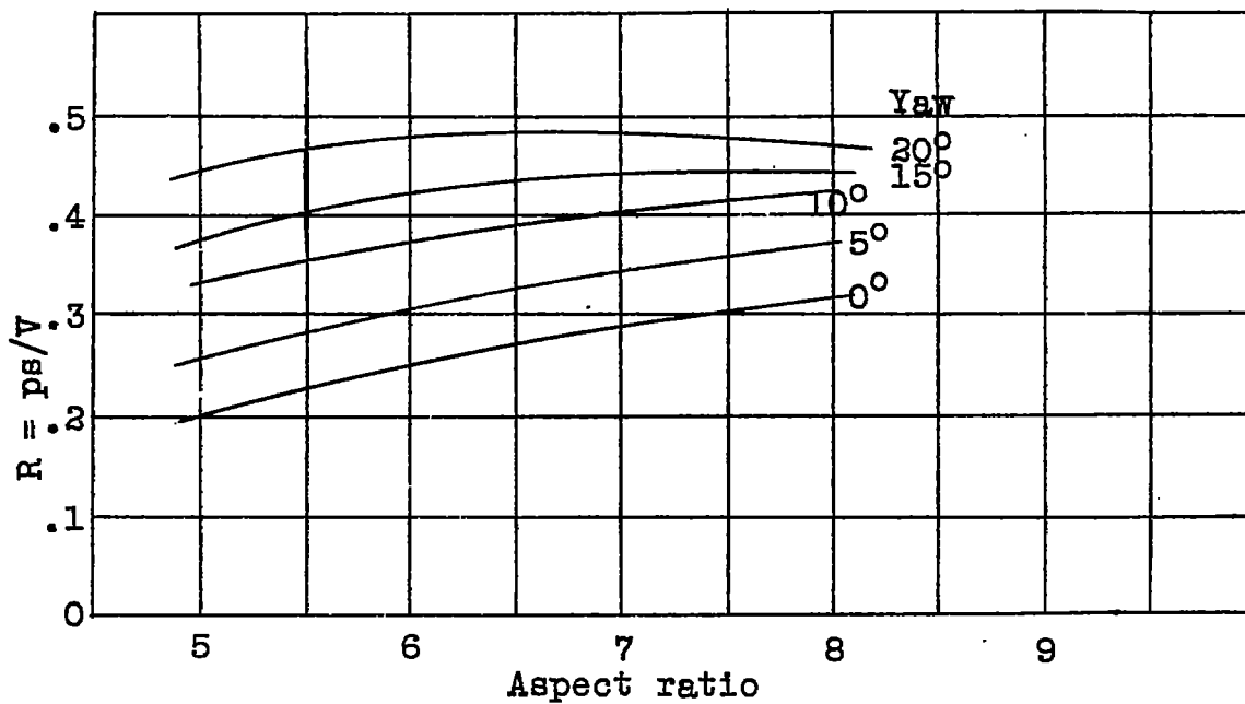
Fig.11 Effect of aspect ratio and yaw on "R". Curves give peak values ( \alpha 20^\circ to 30^\circ )
