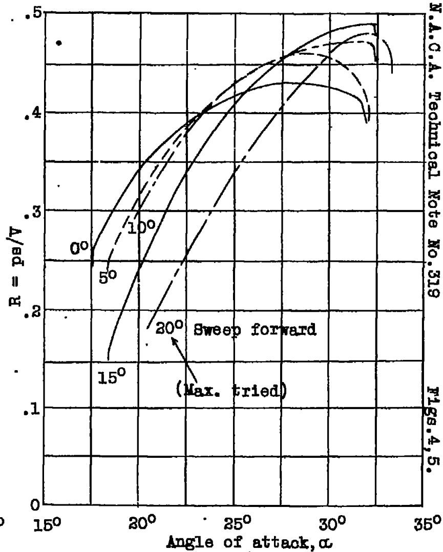
Fig.5 Effect of sweep forward on R.
