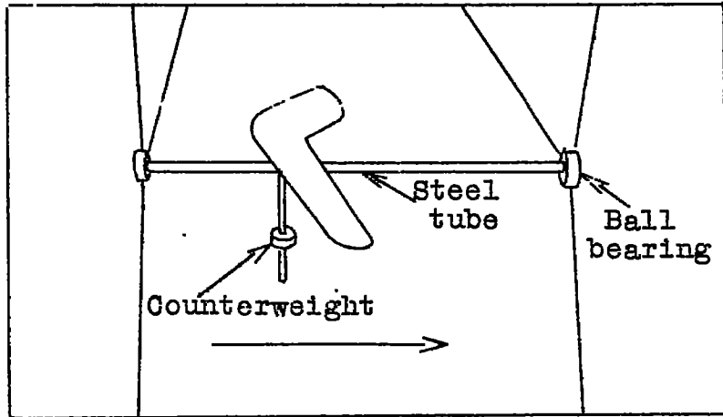
Fig.2 Rotation apparatus, (with sweepback model)
