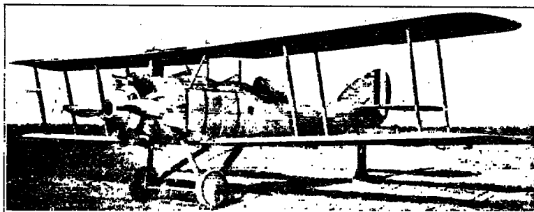
FIG. 1.—UO-1 airplane with Wright J-4 engine and experimental installation of N. A. C. A. Roots type supercharger
