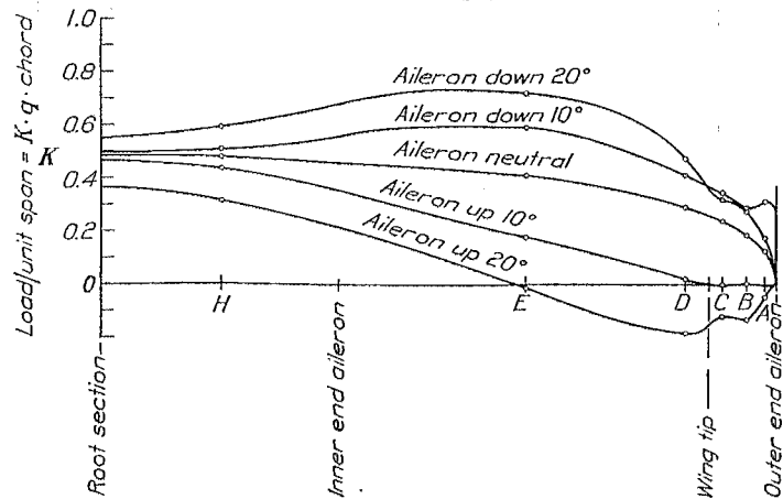
FIG. 9.—Air load distribution along span. Angle of attack 0°
