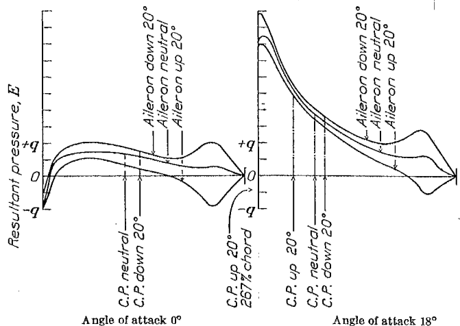
FIG. 8.—Effect of aileron displacement on resultant pressure along chord of section E
