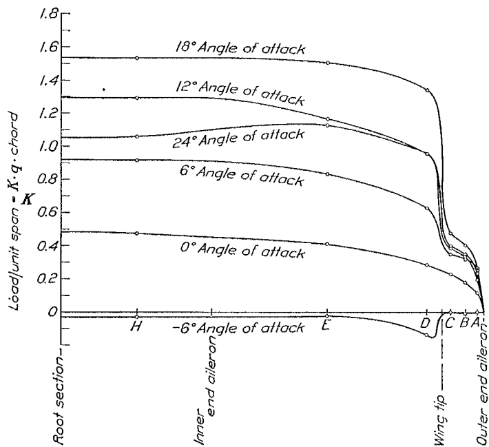
FIG. 7.—Air load distribution along span. Aileron neutral
