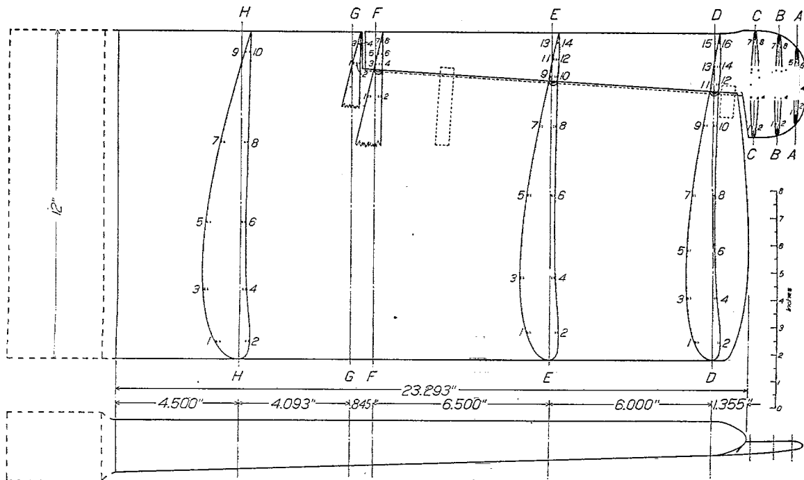
FIG. 1.—Pressure distribution model of the upper wing and aileron of Fokker D-VII Airplane
