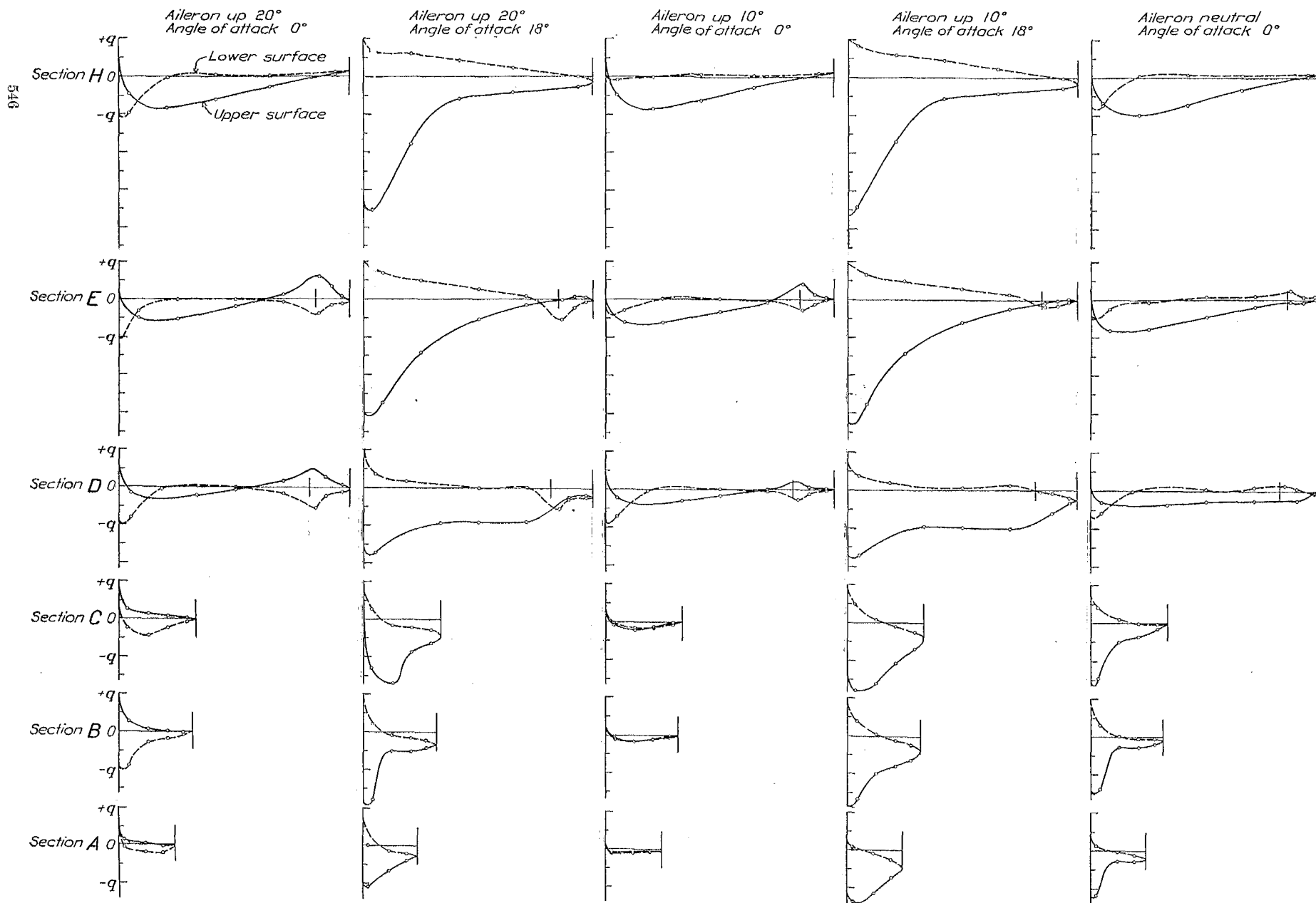
FIG. 5.—Charts of pressure on upper and lower surfaces at test sections, A, B, C, D, E, and H
