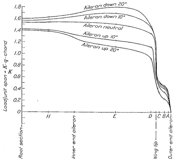
FIG. 10.—Air load distribution along span. Angle of attack 18°
