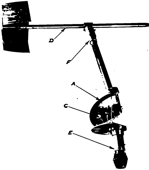
Fig. 1 Angle of attack vane and controlling mechanism.
