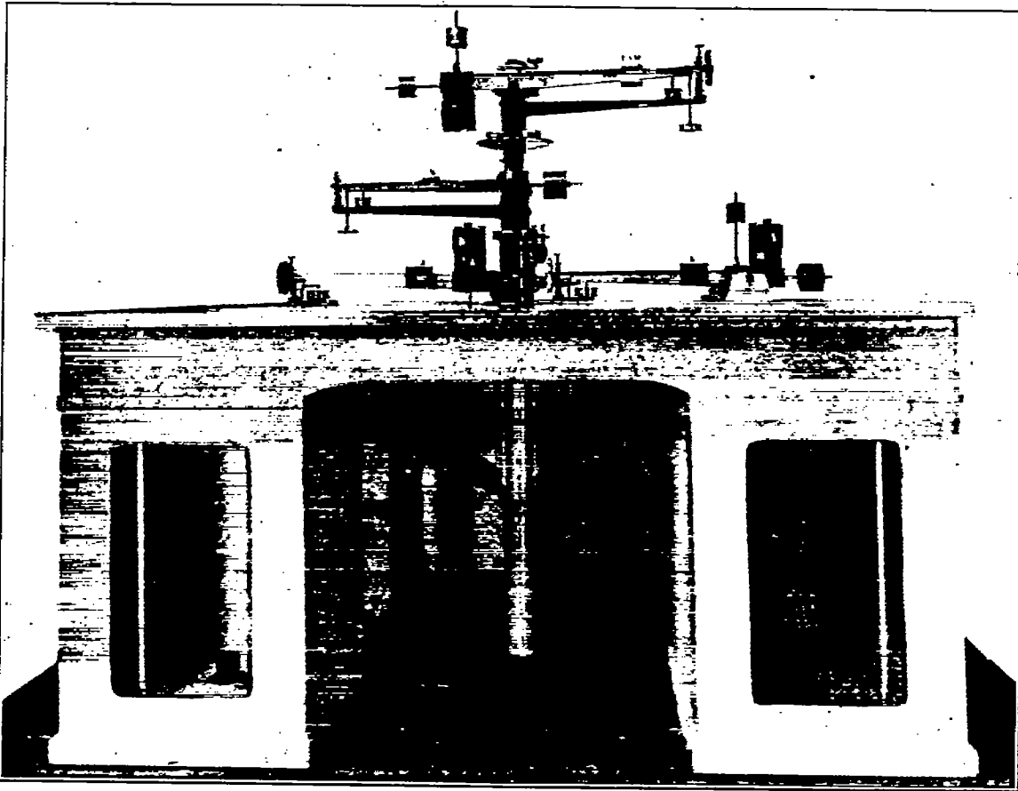
FIG. 2.—Wind balance, front view.
